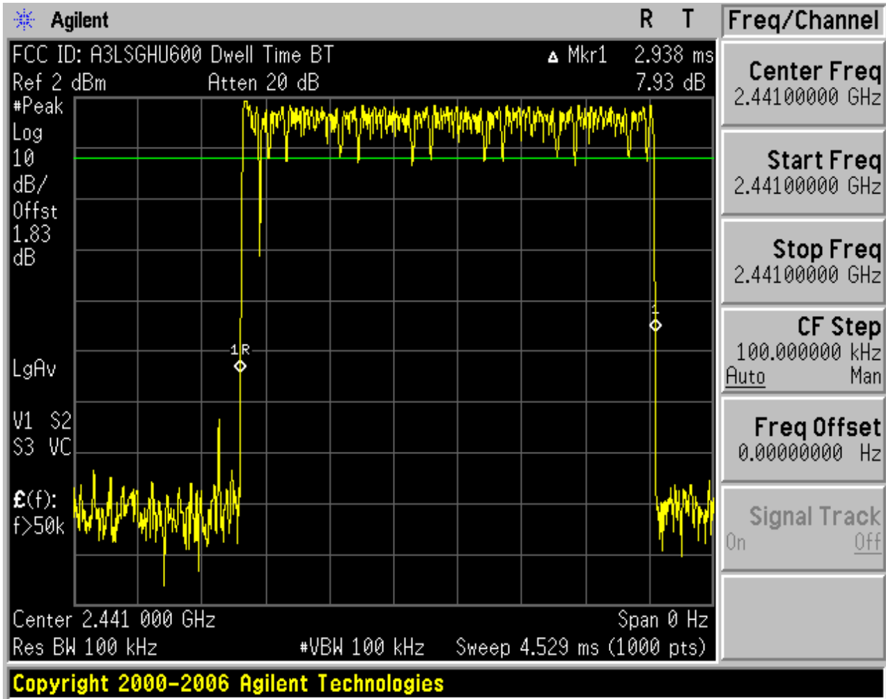
Plot 6-9. Time of Occupancy Plot (Bluetooth)
