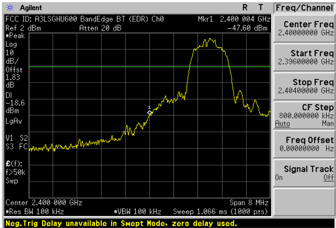
Plot 6-6. Band Edge Plot (Bluetooth 2.0 with Enhanced Data Rate – Ch. 0)
