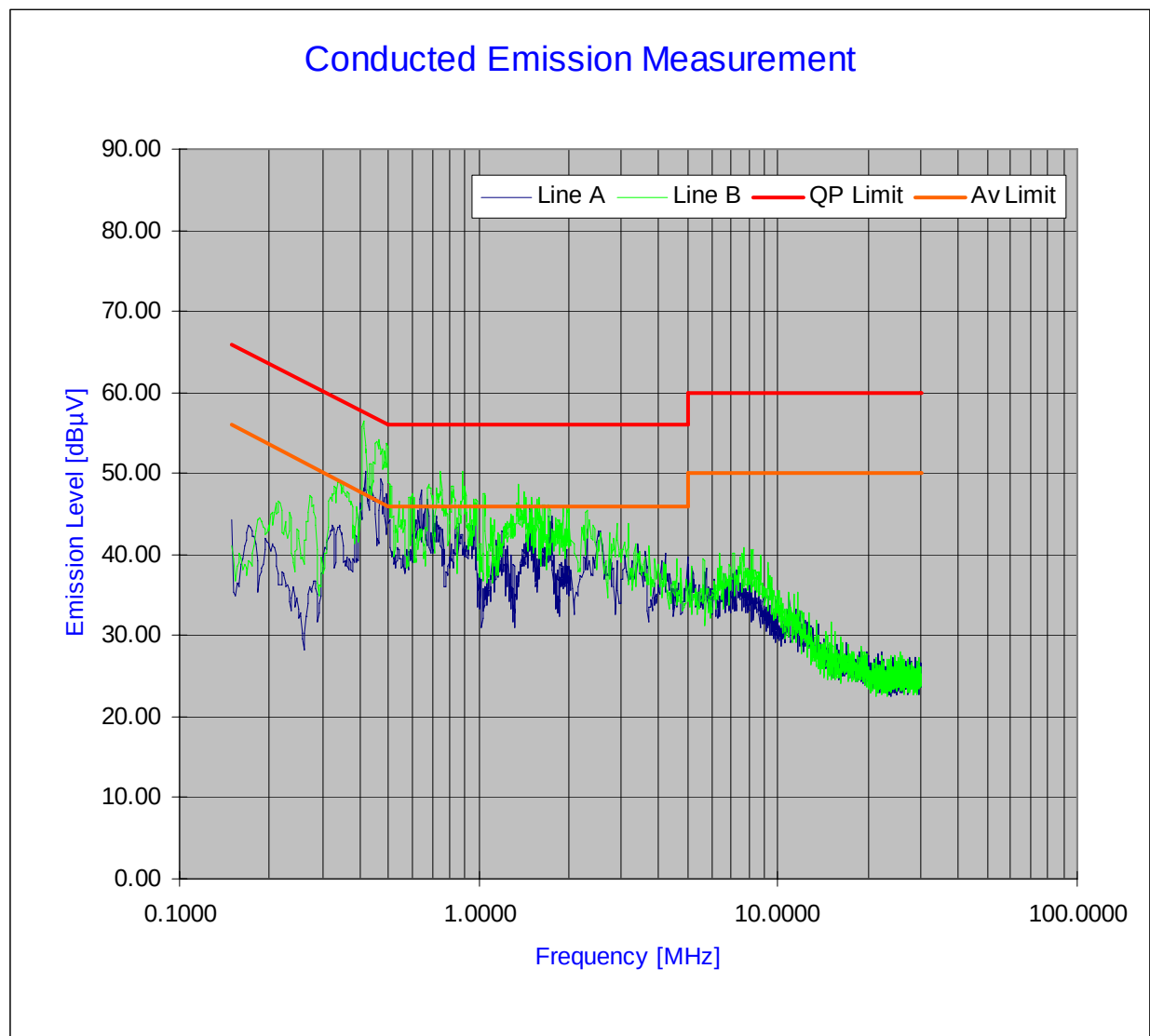
Plot 6-16. Line Conducted Plot with Bluetooth
