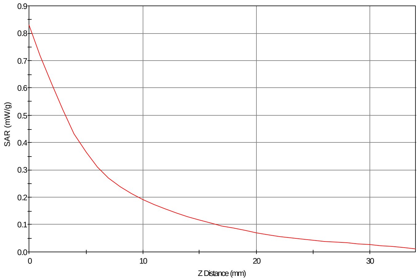
SAR - Z Axis at Hotspot x:-1.0 y:23.0
