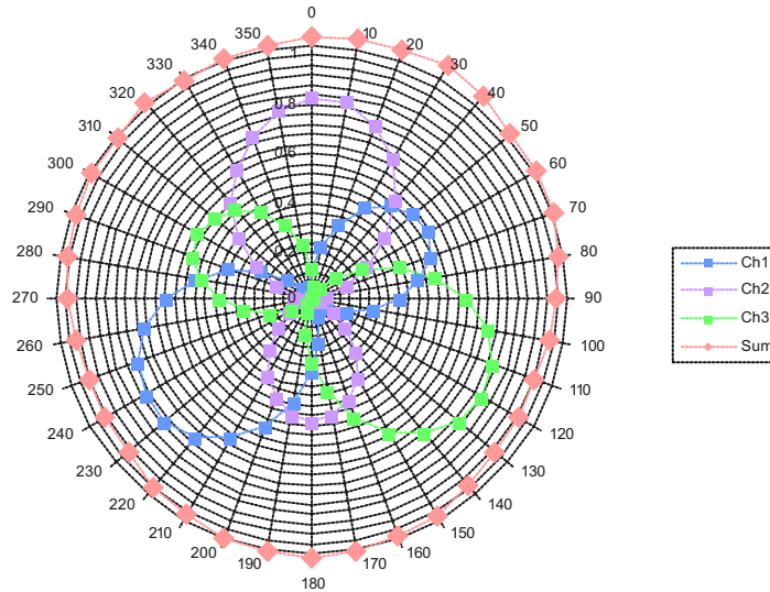
1900 MHz Calibration (PCT005)
