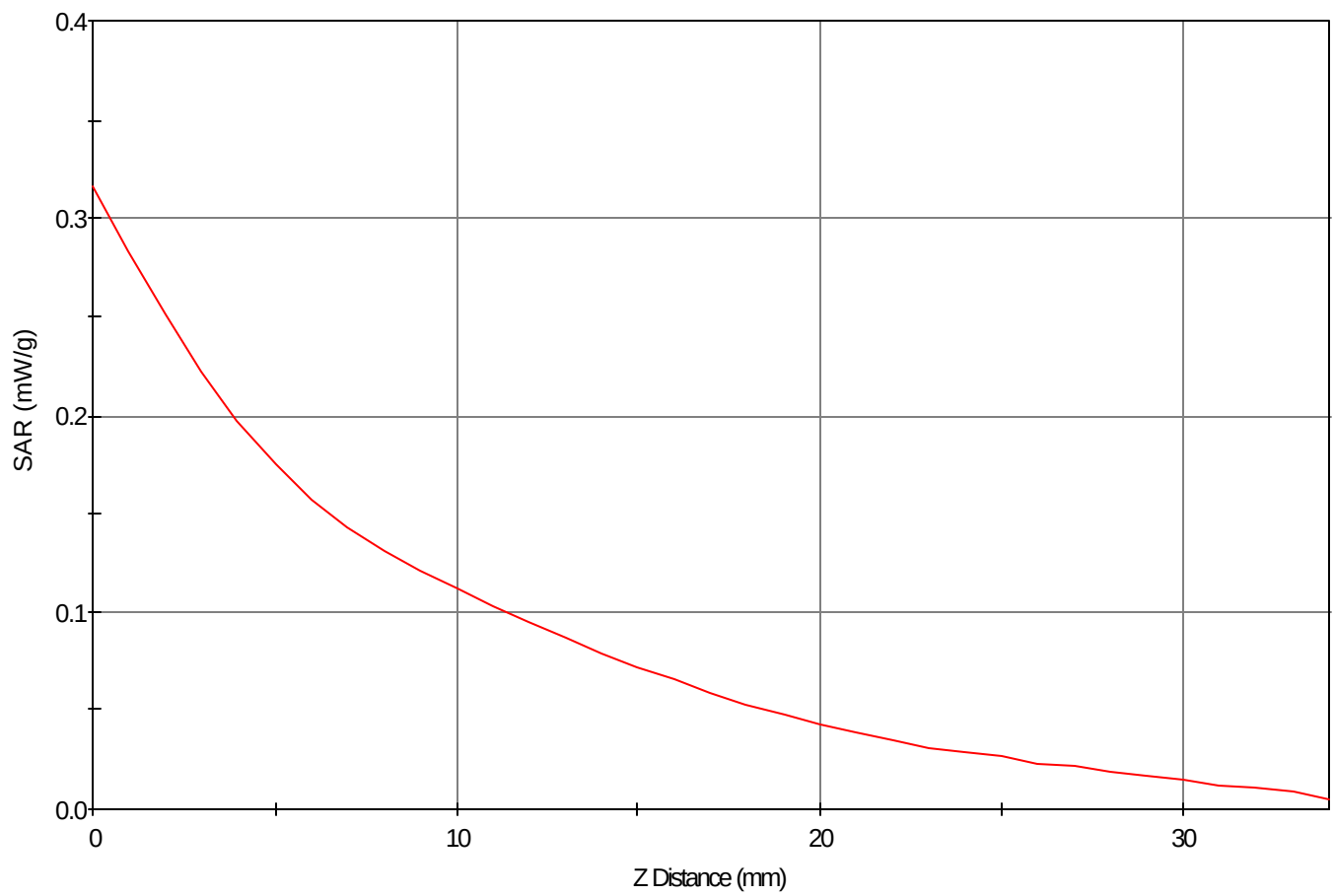
SAR - Z Axis at Hotspot x:38.0 y:4.0
