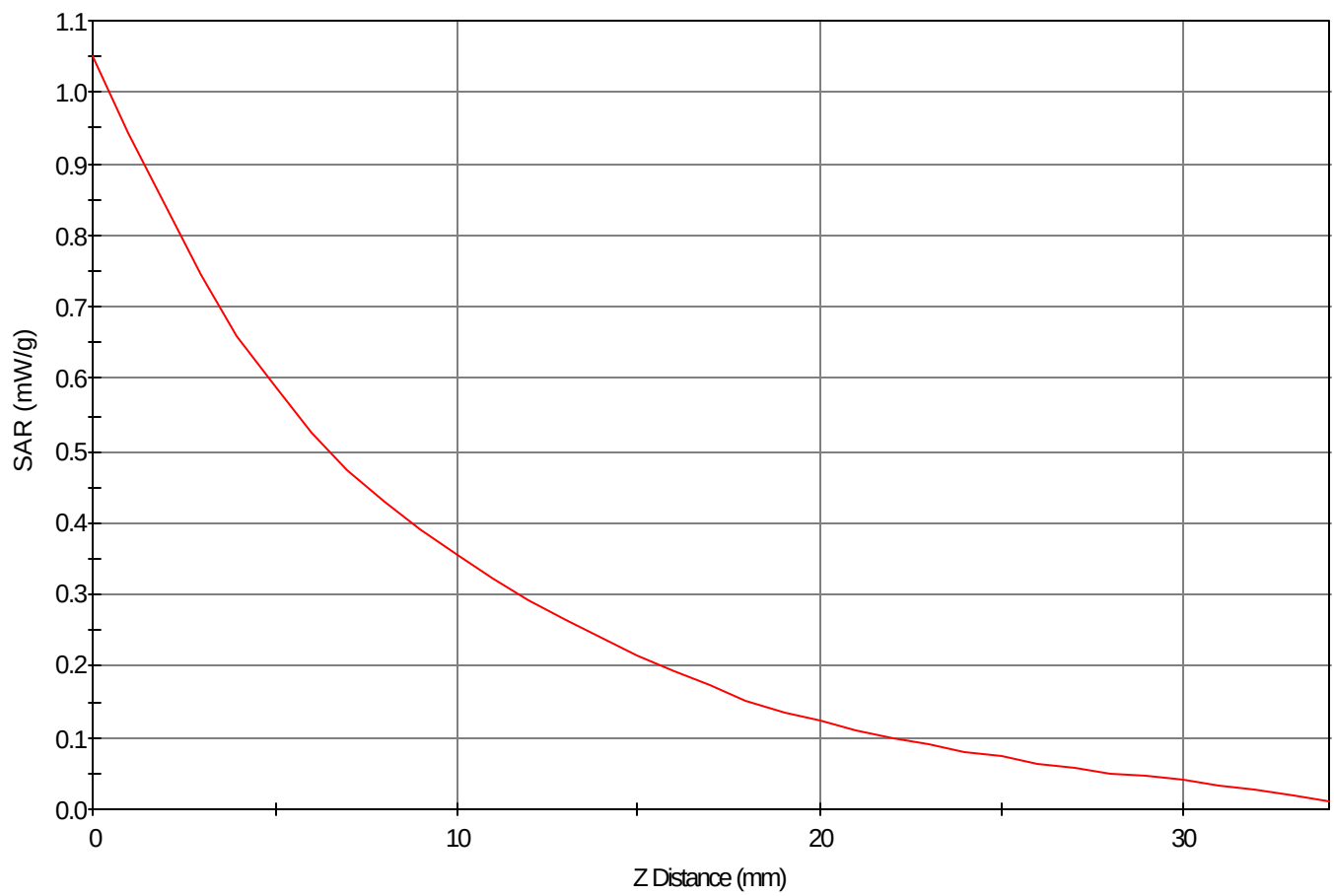
SAR - Z Axis at Hotspot x:63.0 y:13.0
