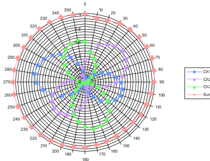
2450 MHz Calibration (PCT005)
