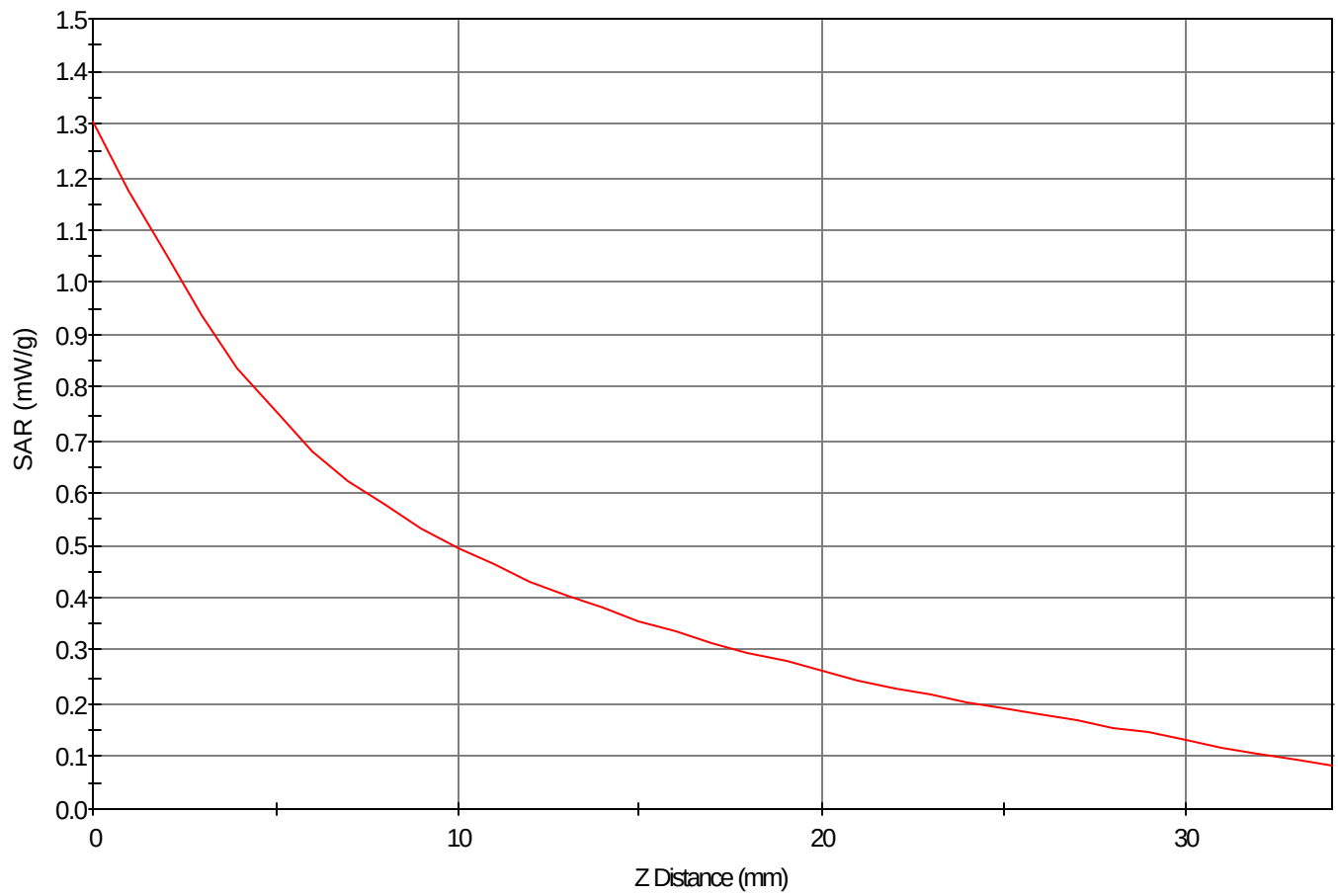
SAR - Z Axis at Hotspot x:80.0 y:5.0
