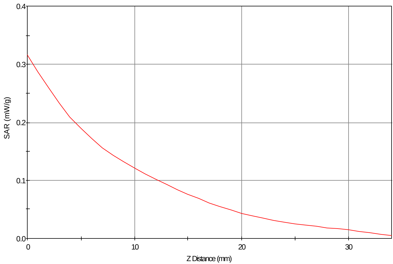
SAR - Z Axis at Hotspot x:16.0 y:9.0
