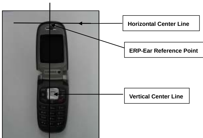
Figure 8.1 Handset Reference Points
