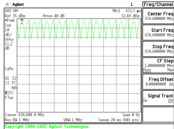
Figure 9-3 GSM850 80% AM Signal
