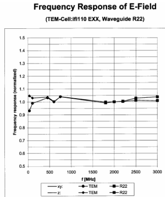
Figure 5-5 E-Field Probe Frequency Response
