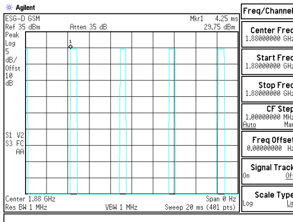
Figure 9-6 PCS GSM Signal
