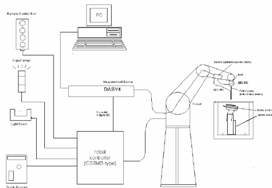
Figure 5-9 SPEAG Robotic System Diagram
