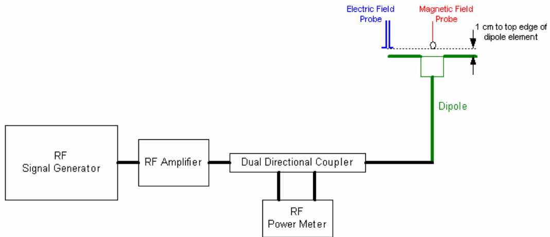
Figure 8-8 System Check Setup
