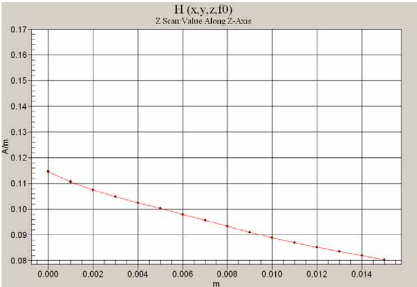
Figure 5-4 Z-Axis Scan at maximum point above a typical wireless device for H-field
