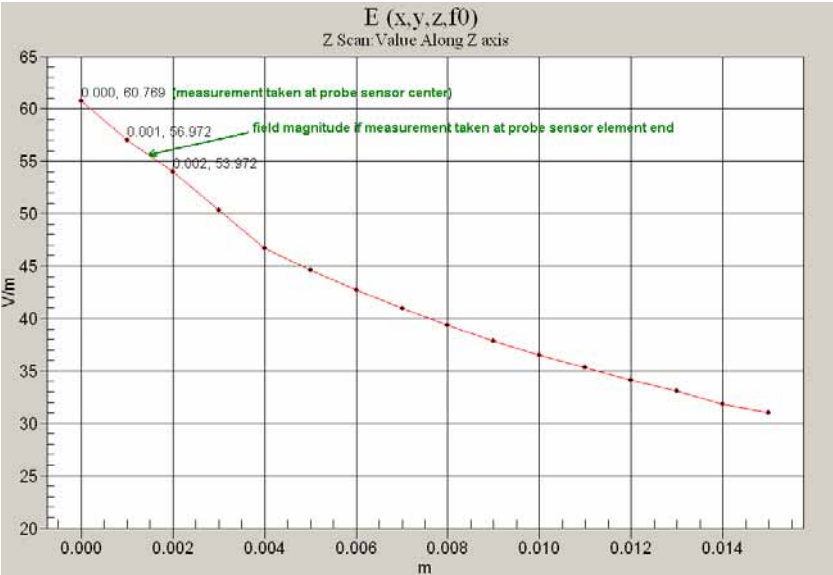
Figure 5-3 Z-axis scan at maximum point above a typical wireless device for E-field
