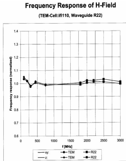
Figure 5-6 H-Field Probe Frequency Response
