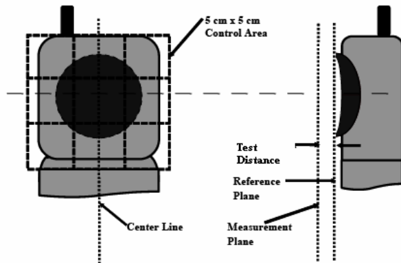
Figure 6-1 E/H-Field Emissions Test Setup Diagram
