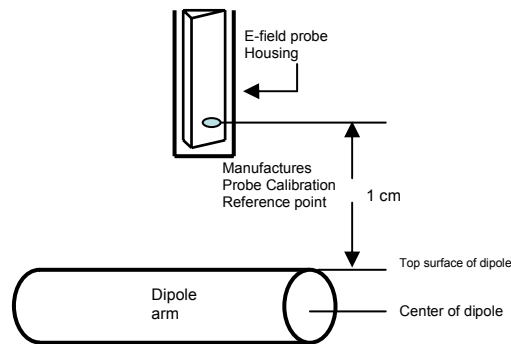
Figure 8-1 Separation Distance from Dipole to Field Probe
