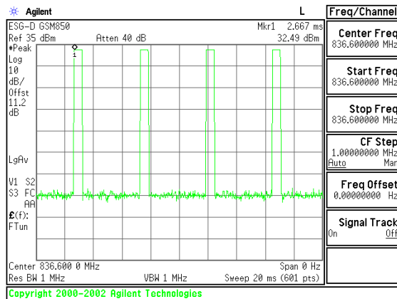
Figure 9-4 GSM850 Signal
