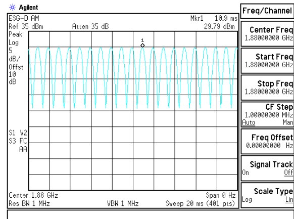
Figure 9-7 PCS 80% AM Signal
