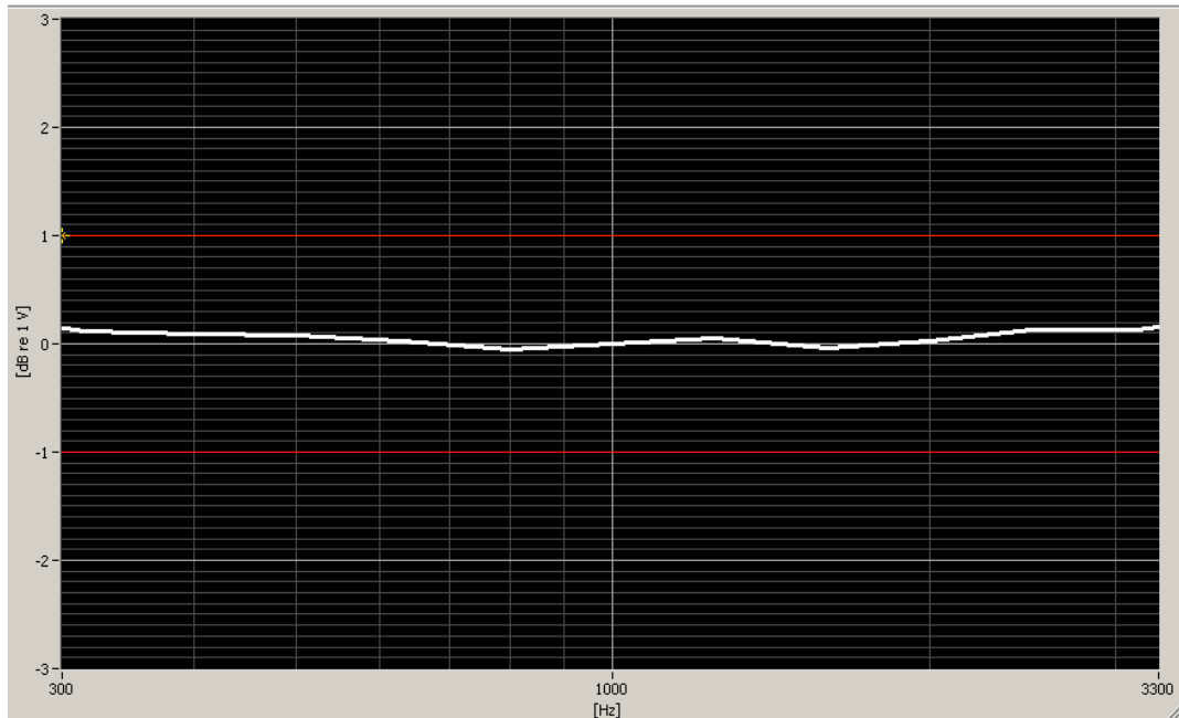
Figure 6-3 Helmholtz Coil Validation for Frequency Response
