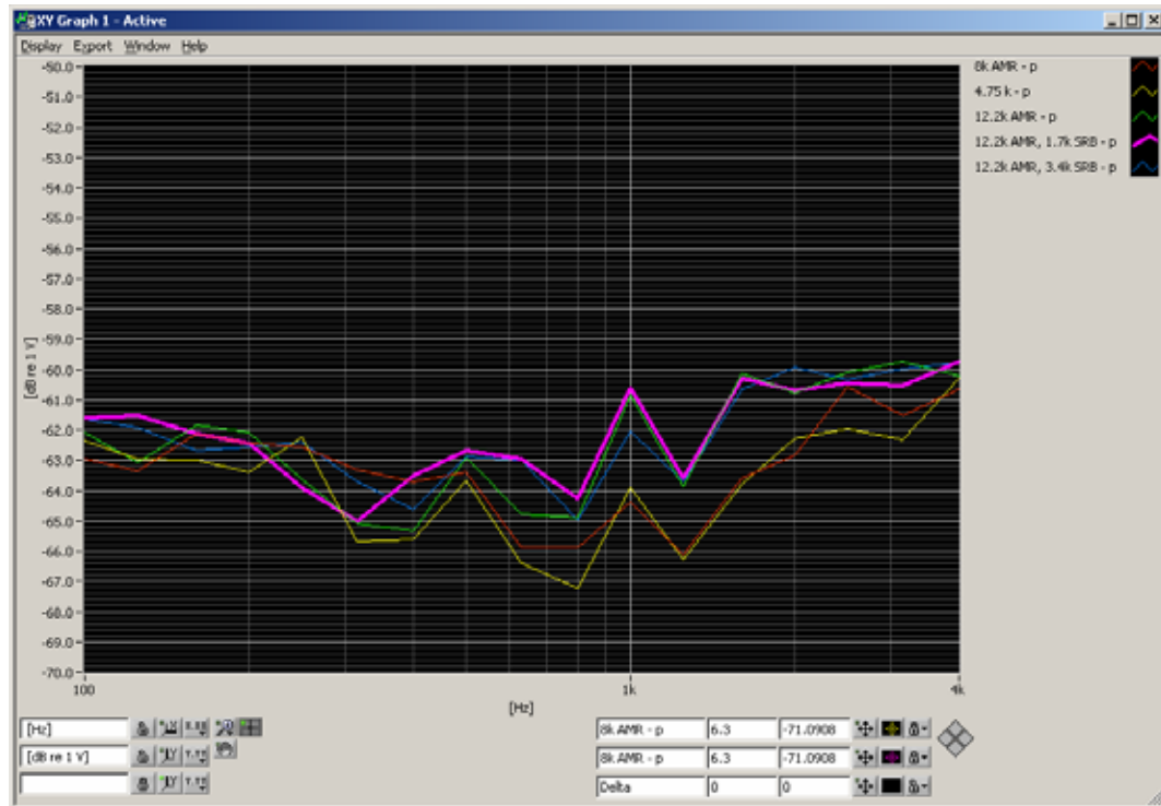
Figure 7-1 WCDMA Audio Band Magnetic Noise
