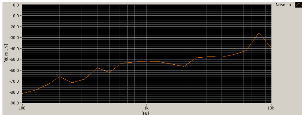
Figure 6-2 Worst-case ABM2 Plot for WD
