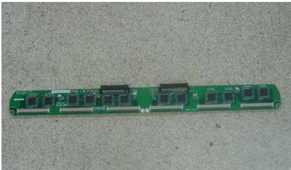
YB board top view
