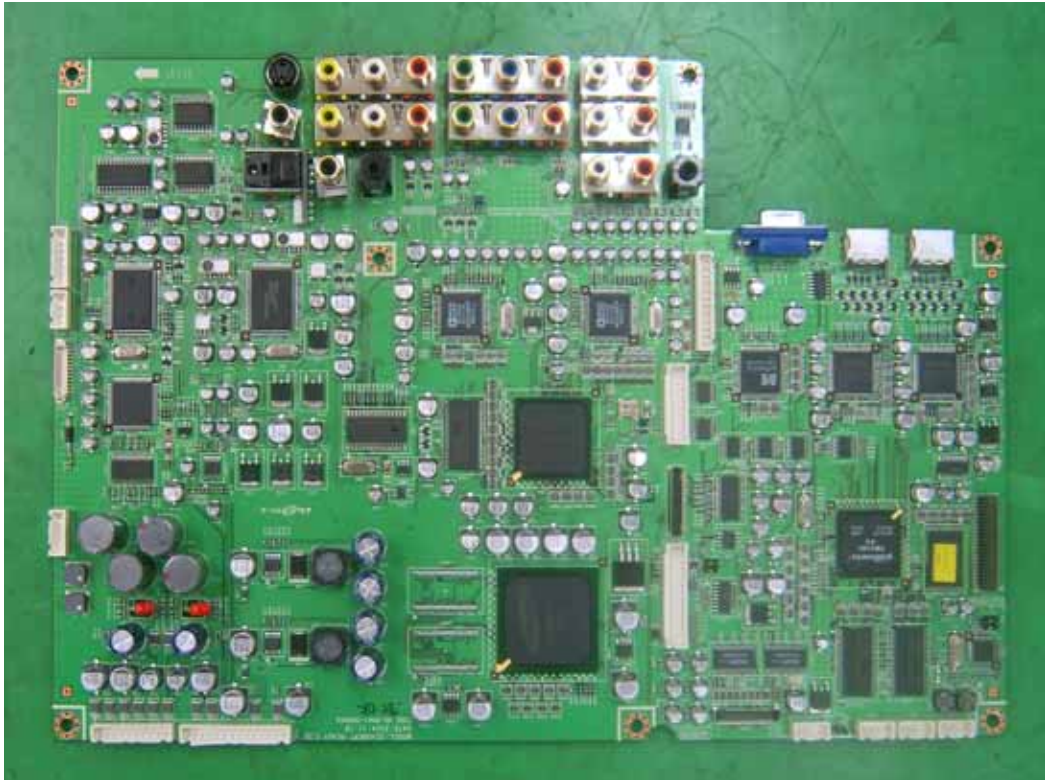
Visual board-1 top view
