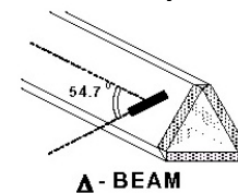
Fig 4-3 Triangular Probe Configuration
