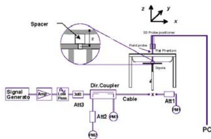
Fig 12-3 System Verification Setup Diagram
