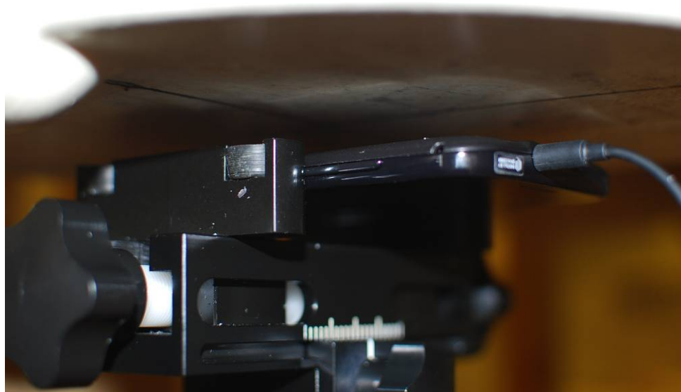
SAR Test Setup Photo 11 – Body-Worn Back at 1.0 cm
