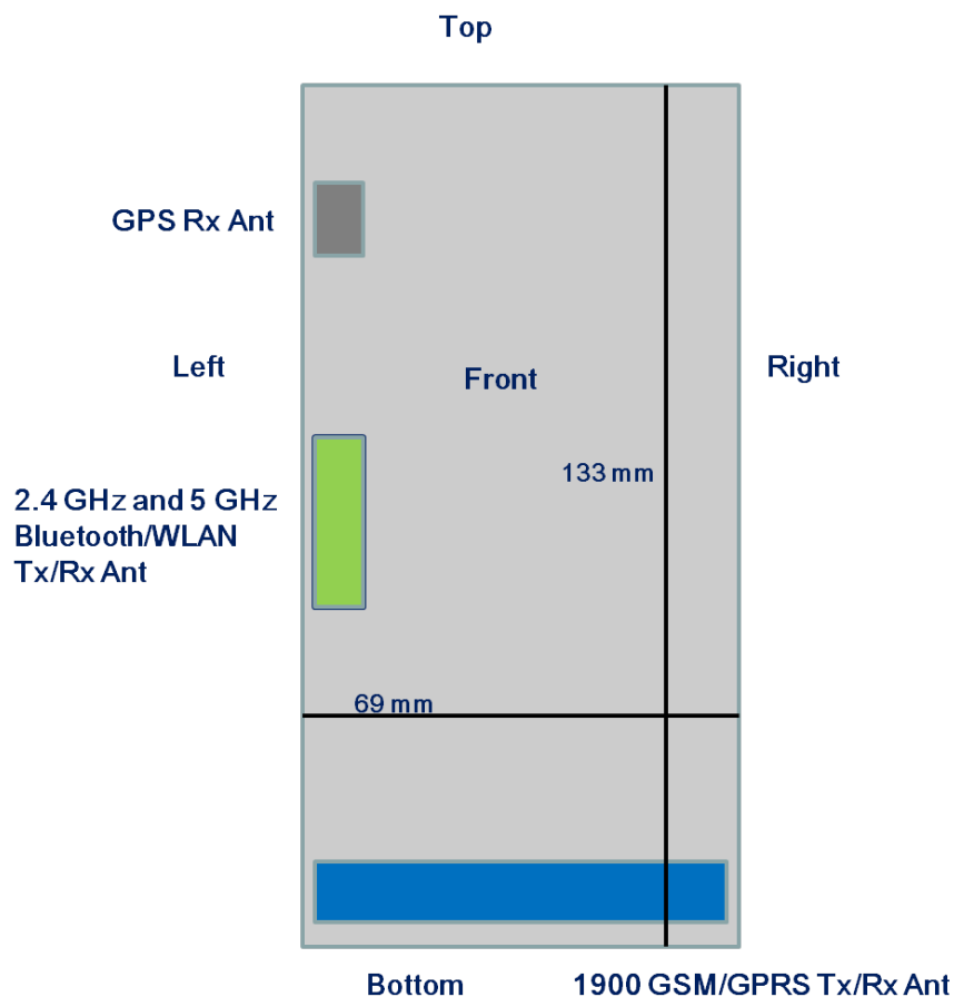
Figure 13-1 Identification of Sides for SAR Testing
