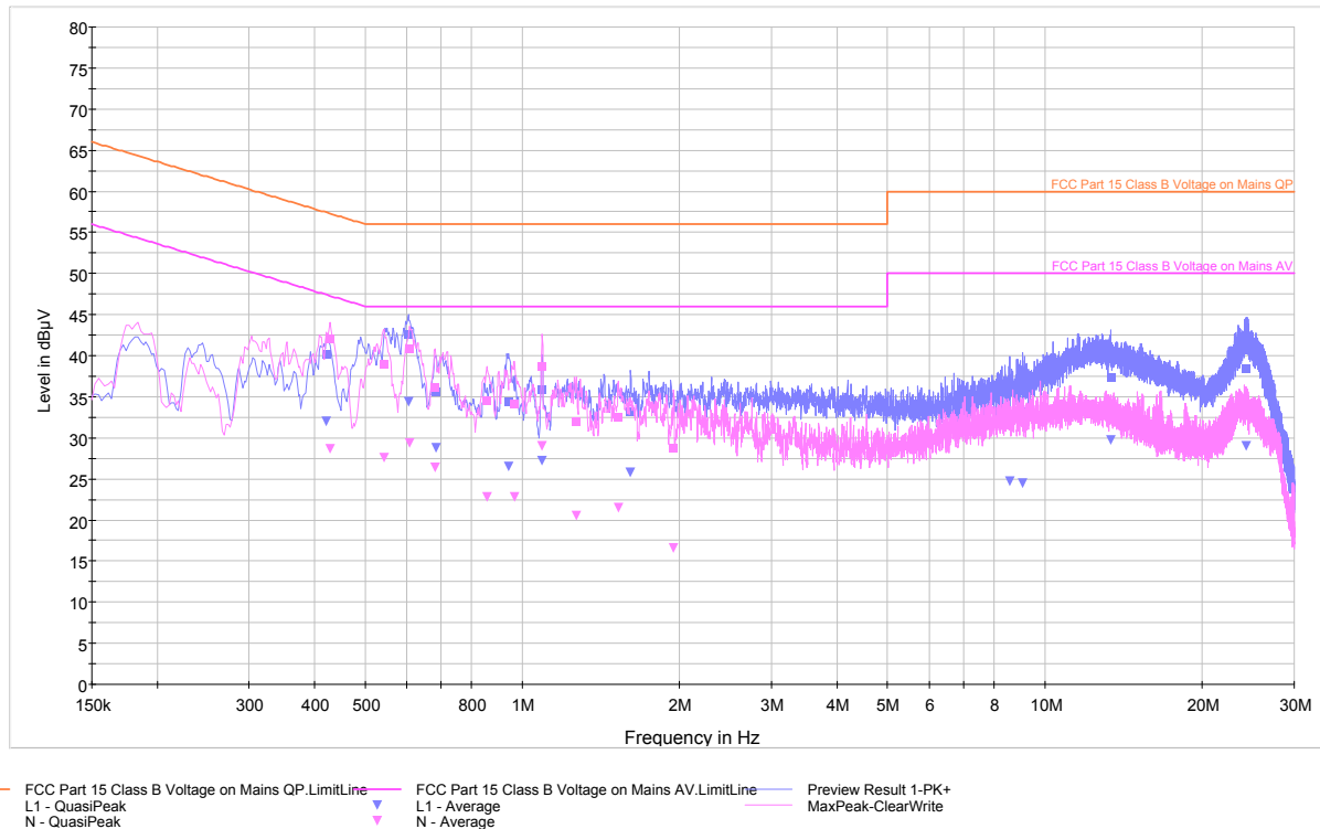
Plot 8-1. Line-Conducted Test Plot
