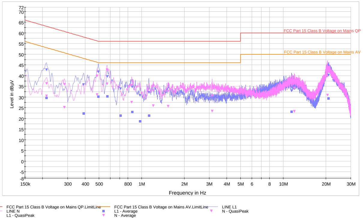
Plot 6-55. Line Conducted Plot with 802.11a (UNII Band 1)
