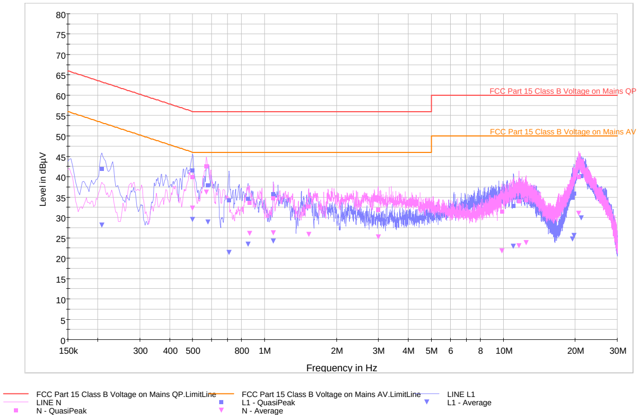
Plot 6-57. Line Conducted Plot with 802.11a (UNII Band 3)
