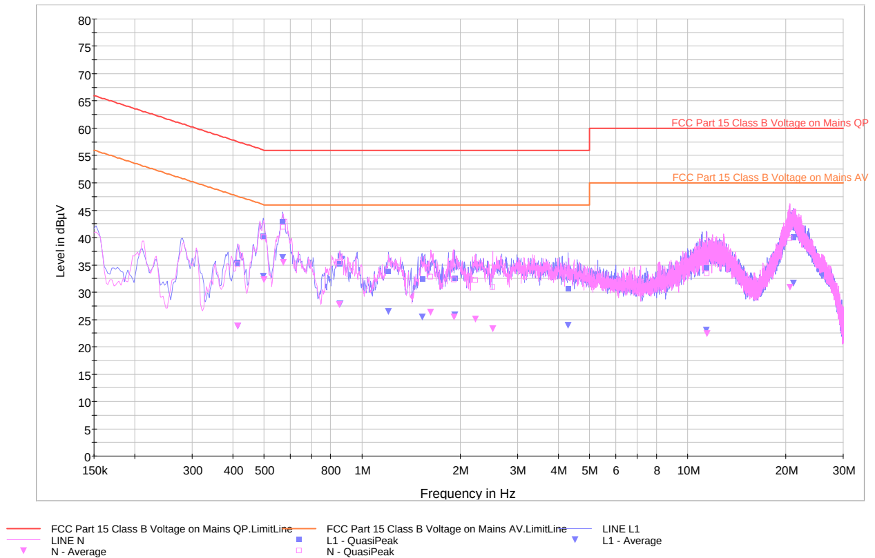
Plot 6-56. Line Conducted Plot with 802.11a (UNII Band 2)
