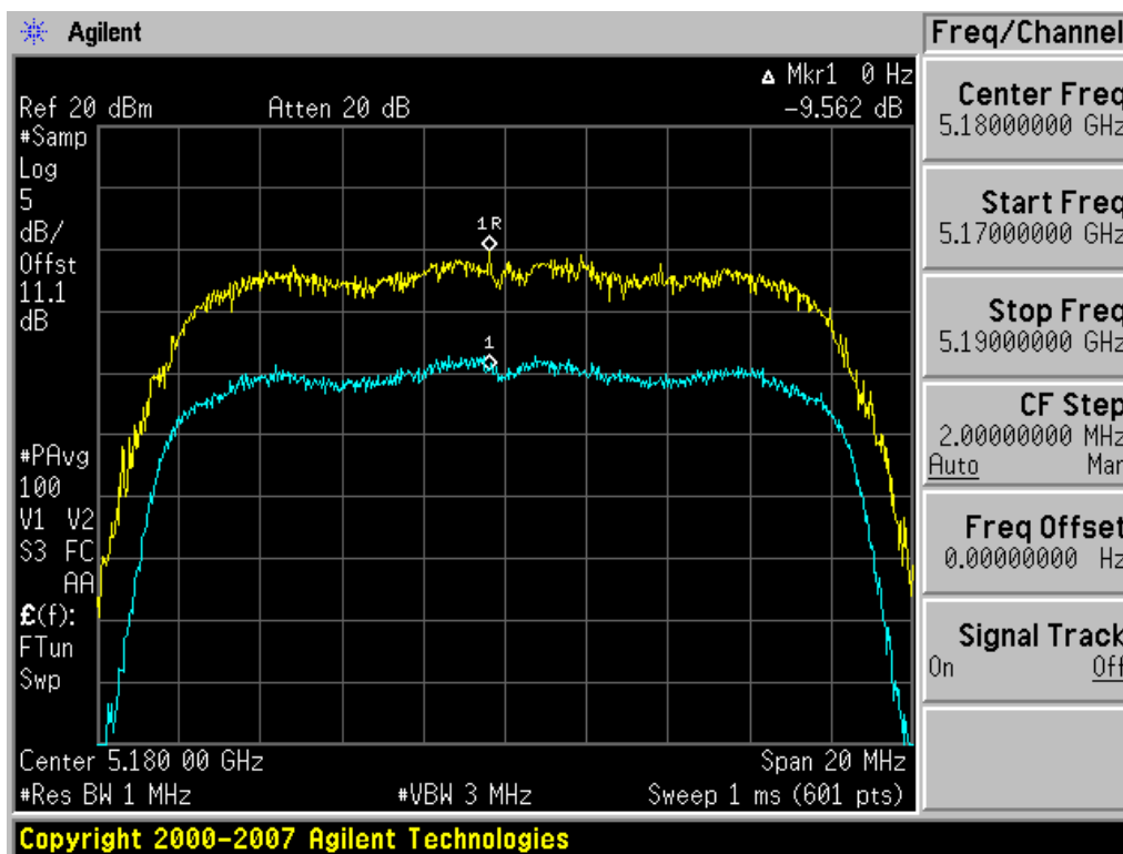
Plot 6-37. Peak Excursion Ratio Plot (802.11a (UNII Band 1) – Ch. 36)
