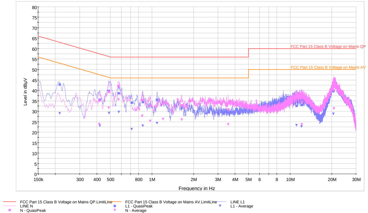
Plot 6-59. Line Conducted Plot with 802.11n (UNII Band 2)
