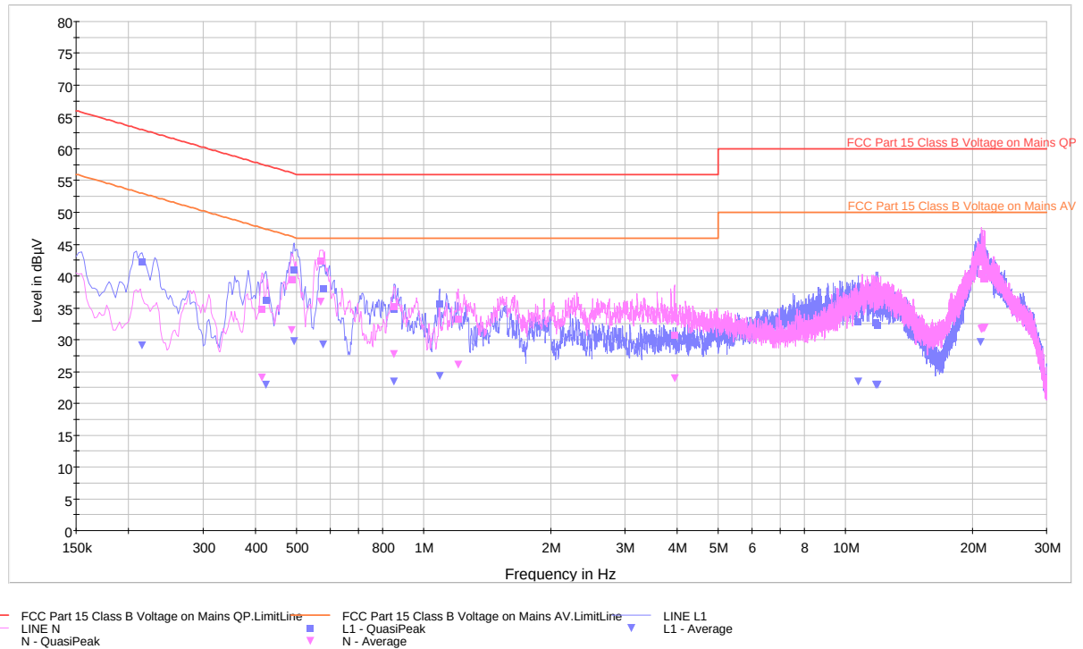
Plot 6-58. Line Conducted Plot with 802.11n (UNII Band 1)
