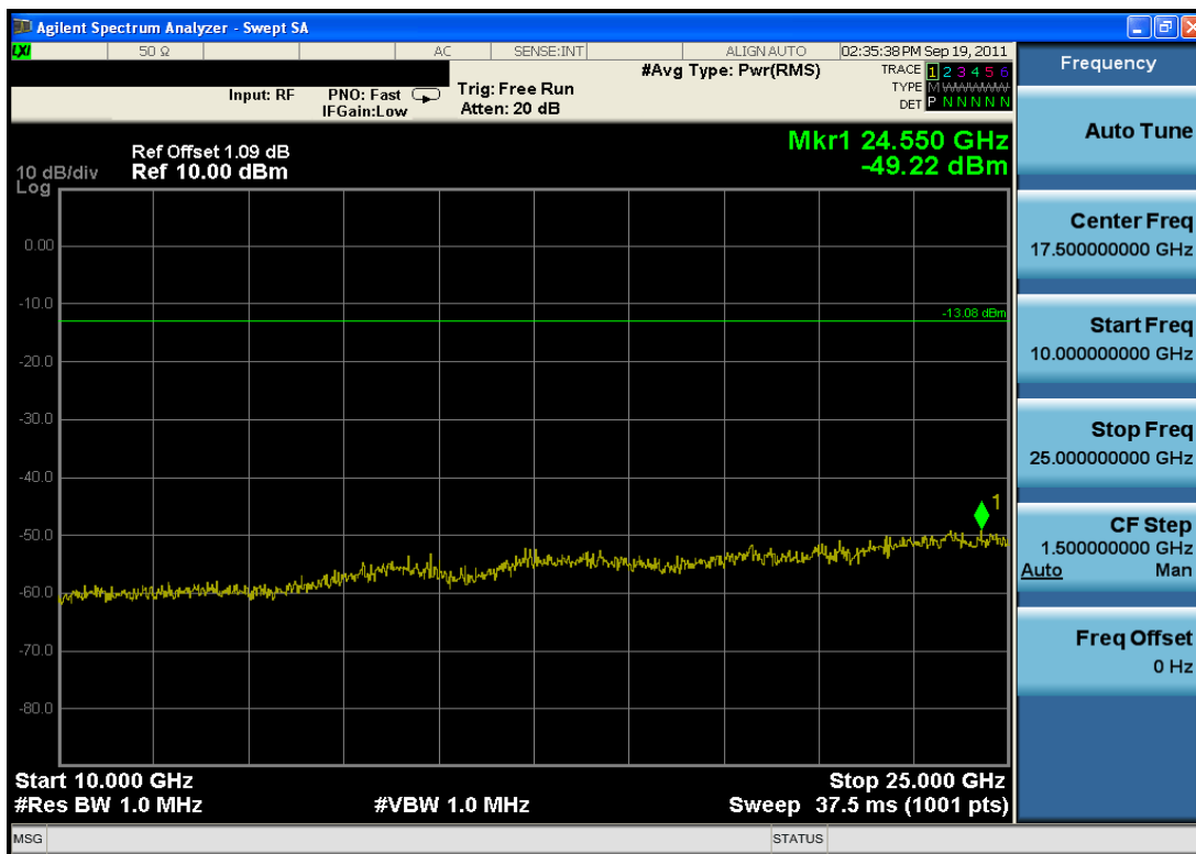
Plot 6-17. Conducted Spurious Plot (Bluetooth, 3Mbps – Ch. 0)
