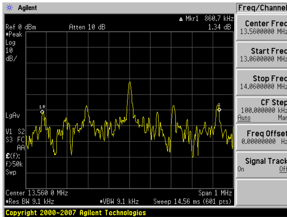
Figure 8-2. Occupied Bandwidth Plot
