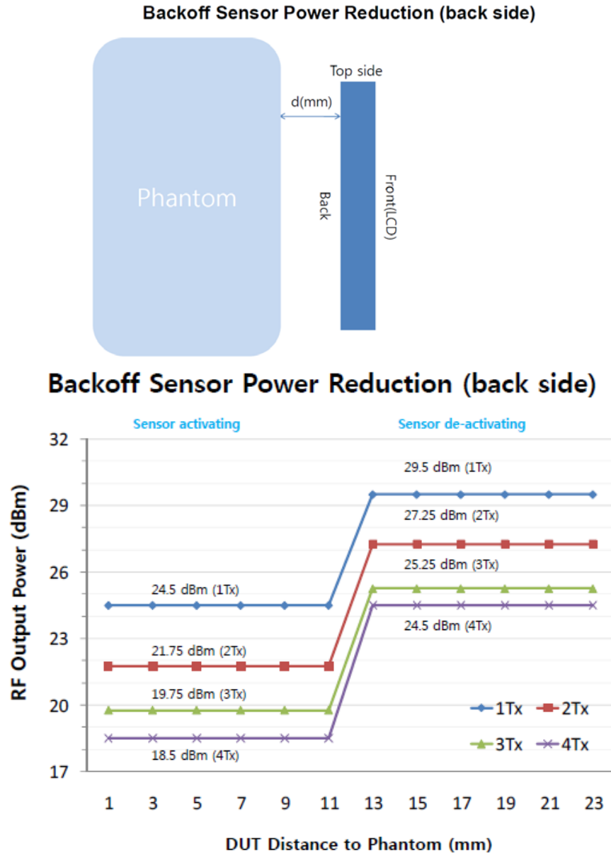
Figure 9-4 GPRS (GMSK) 1900 Back off Power Reduction Graph - Back Side
