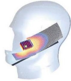
Figure 7-1 Sample SAR Area Scan
