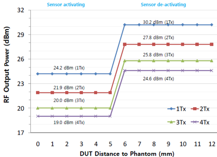
Figure 9-5 GPRS Back off Power Reduction Graph - Top at 0° Angle
