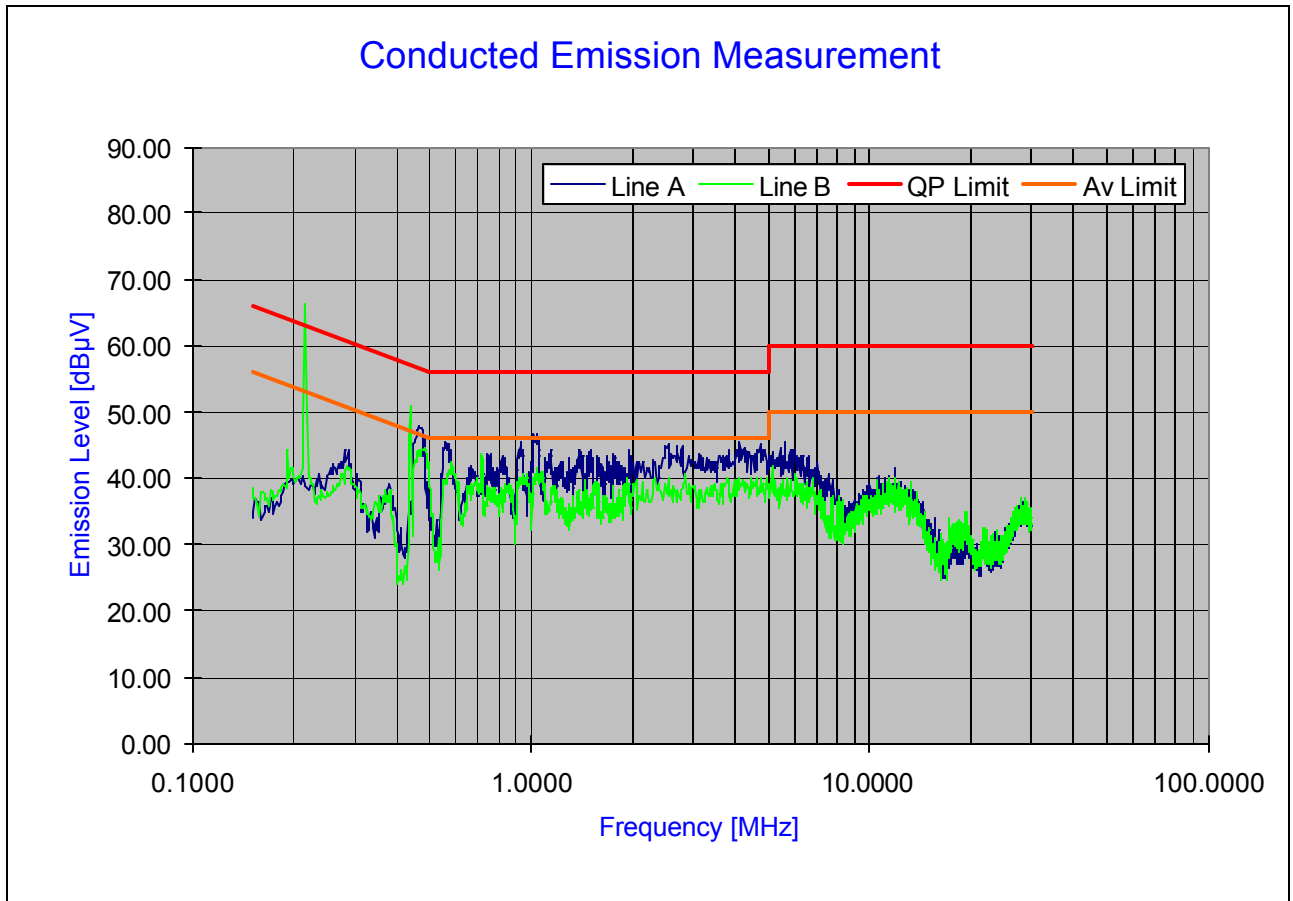
Plot 6-57. Line Conducted Plot with 802.11n (5.8GHz)
