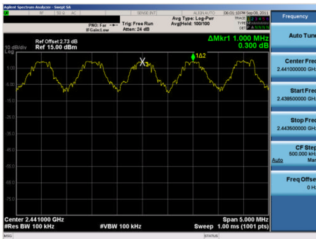
Plot 6-12. Channel Spacing Plot (Bluetooth)
