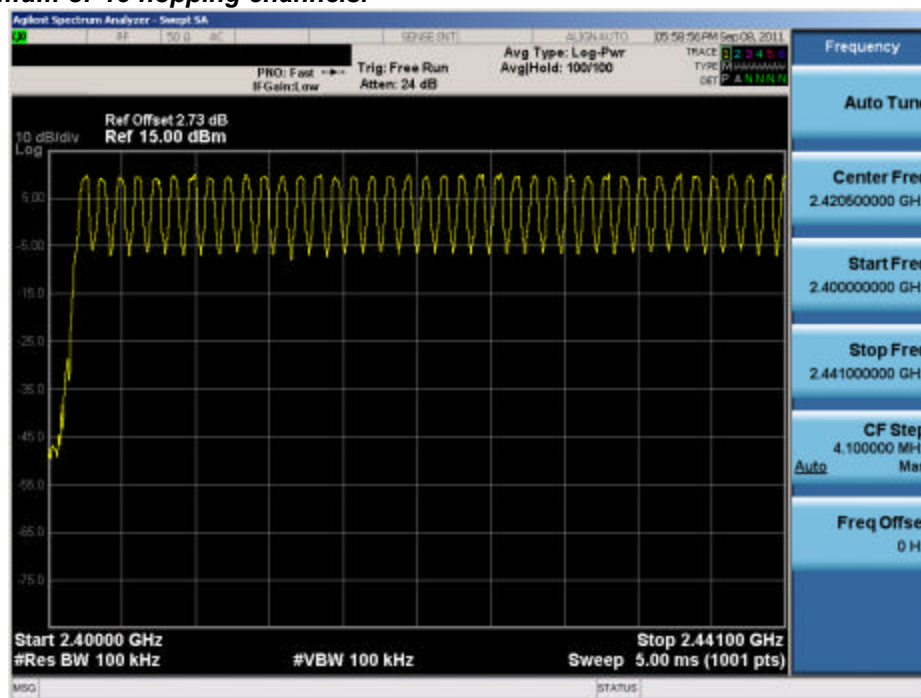
Plot 6-14. Low End Spectrum Channel Hopping Plot (Bluetooth)
