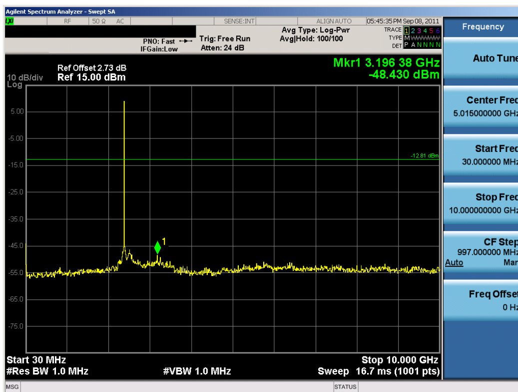
Plot 6-16. Conducted Spurious Plot (Bluetooth, 3Mbps – Ch. 0)
