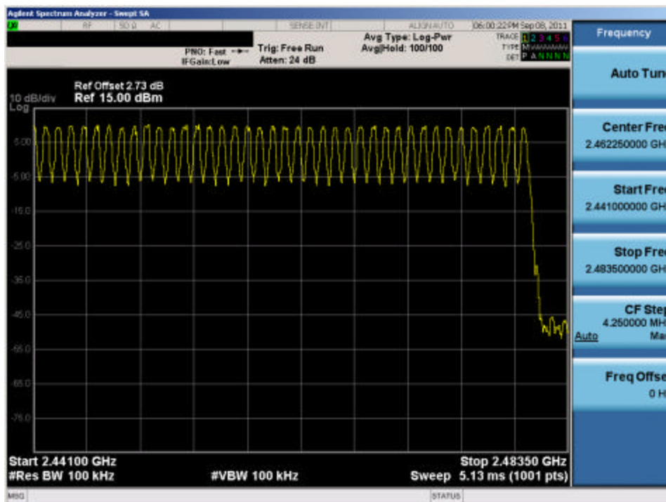
Plot 6-15. High End Spectrum Channel Hopping Plot (Bluetooth)
