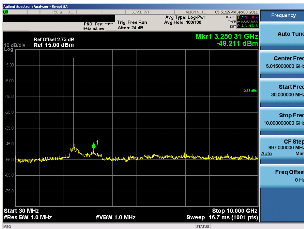
Plot 6-18. Conducted Spurious Plot (Bluetooth, 3Mbps – Ch. 39)
