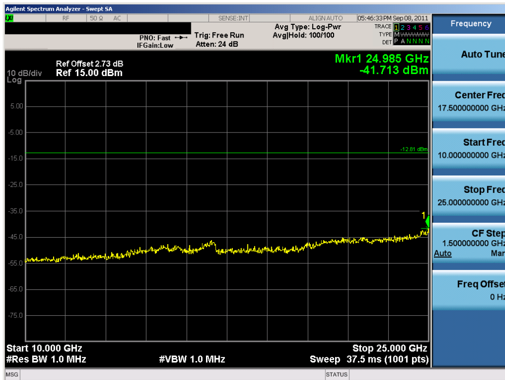
Plot 6-17. Conducted Spurious Plot (Bluetooth, 3Mbps – Ch. 0)
