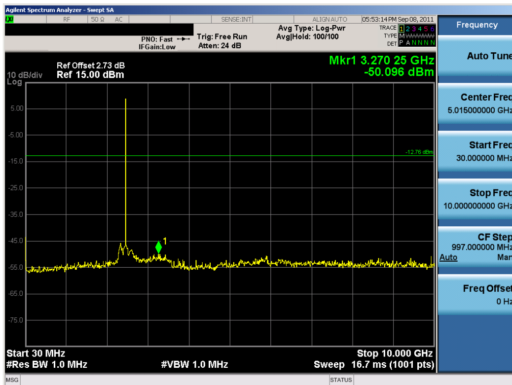
Plot 6-20. Conducted Spurious Plot (Bluetooth, 3Mbps – Ch. 78)
