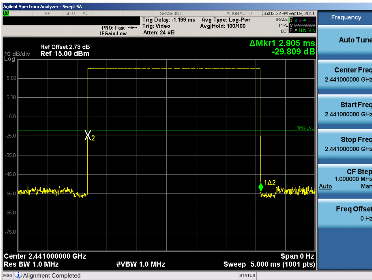
Plot 6-13. Time of Occupancy Plot (Bluetooth)
