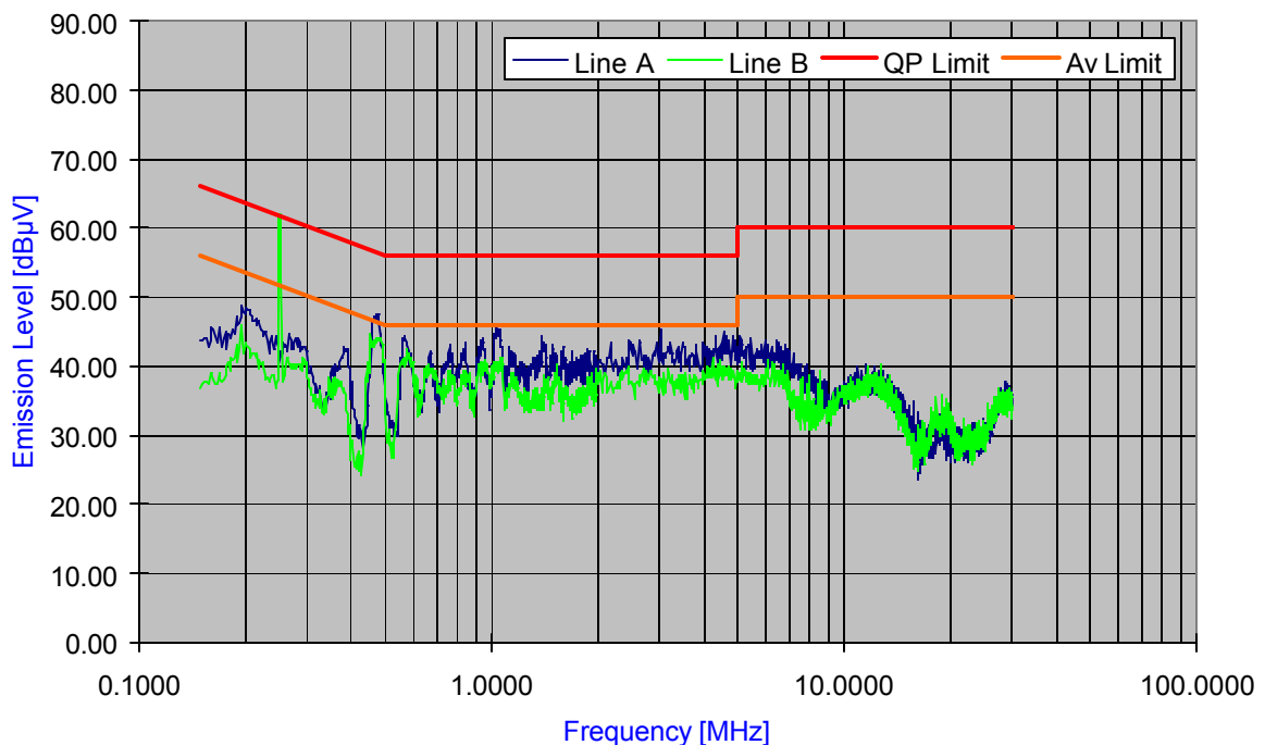
Plot 6-22. Line Conducted Plot with Bluetooth
