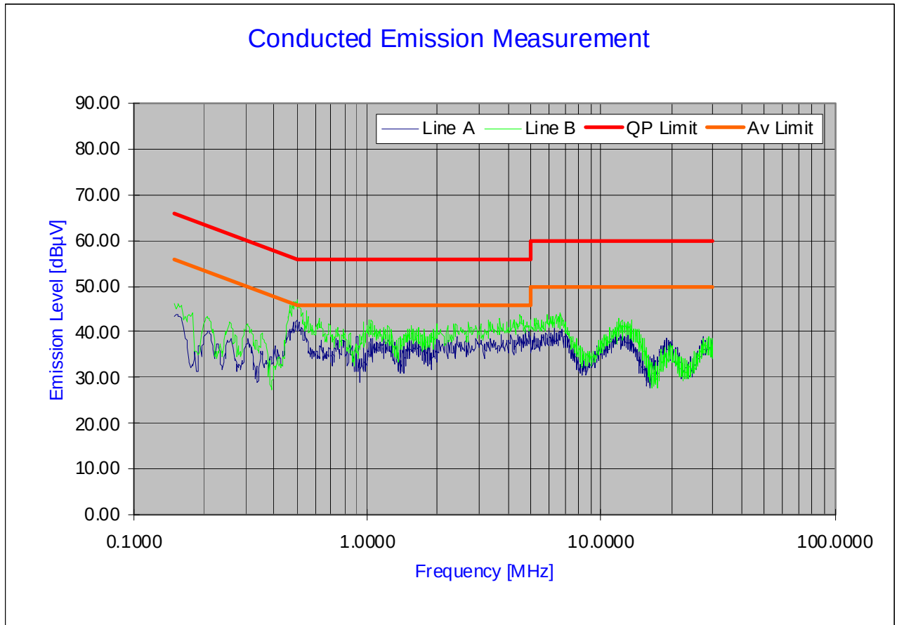
Plot 6-59. Line Conducted Plot with 802.11a
