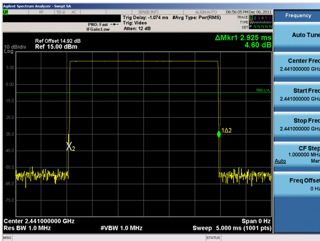
Plot 6-13. Time of Occupancy Plot (Bluetooth)
