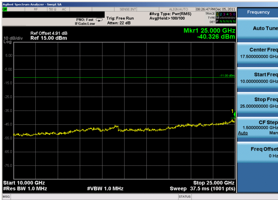
Plot 6-19. Conducted Spurious Plot (Bluetooth, 1Mbps – Ch. 39)
