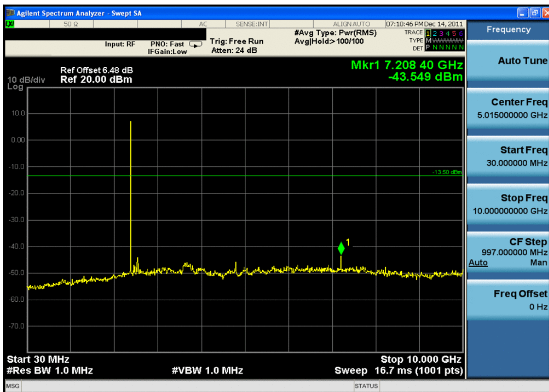
Plot 6-16. Conducted Spurious Plot (Bluetooth, 1Mbps – Ch. 0)
