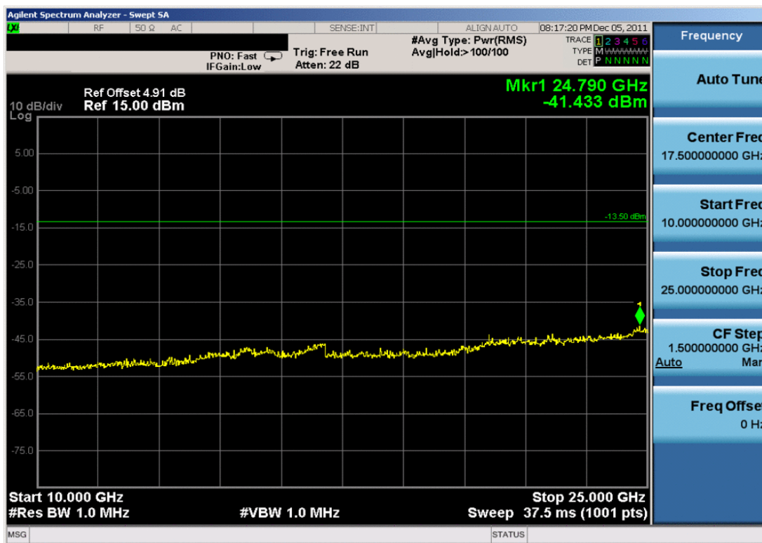
Plot 6-17. Conducted Spurious Plot (Bluetooth, 1Mbps – Ch. 0)
