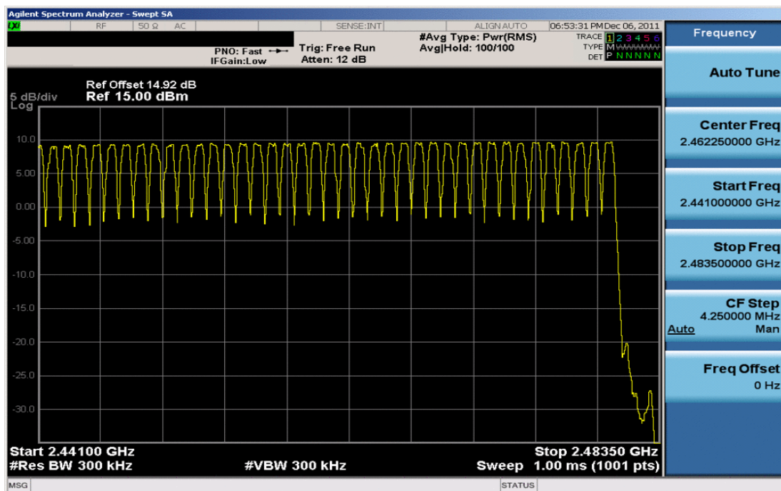
Plot 6-15. High End Spectrum Channel Hopping Plot (Bluetooth)
