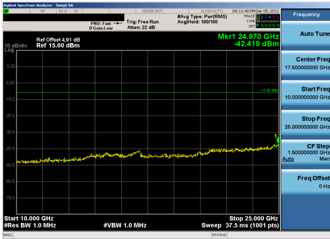
Plot 6-21. Conducted Spurious Plot (Bluetooth, 1Mbps – Ch. 78)
