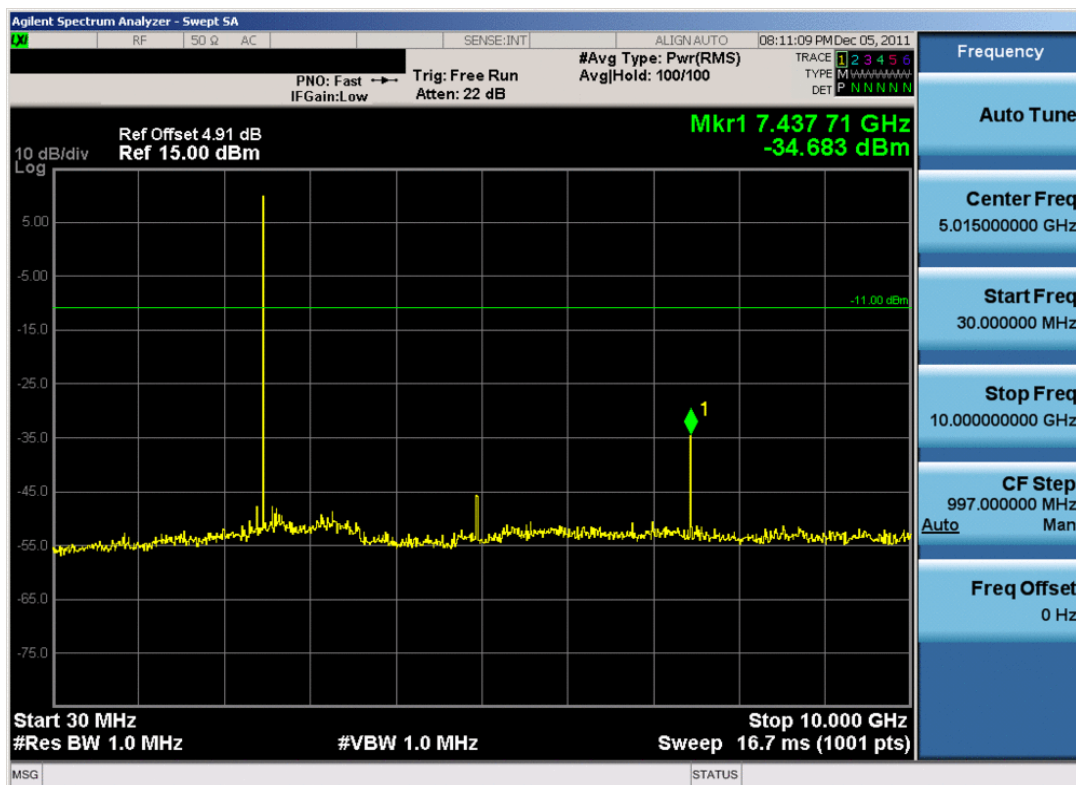
Plot 6-20. Conducted Spurious Plot (Bluetooth, 1Mbps – Ch. 78)
