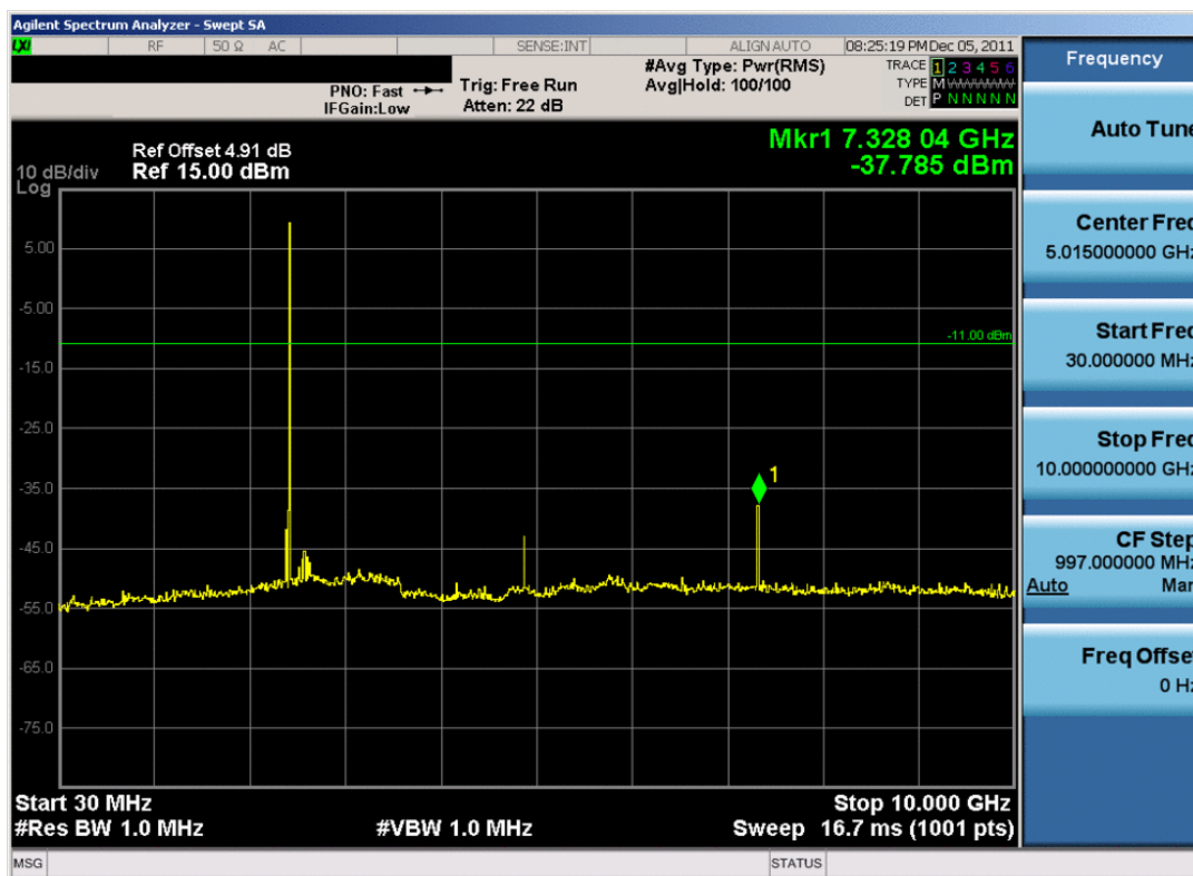
Plot 6-18. Conducted Spurious Plot (Bluetooth, 1Mbps – Ch. 39)
