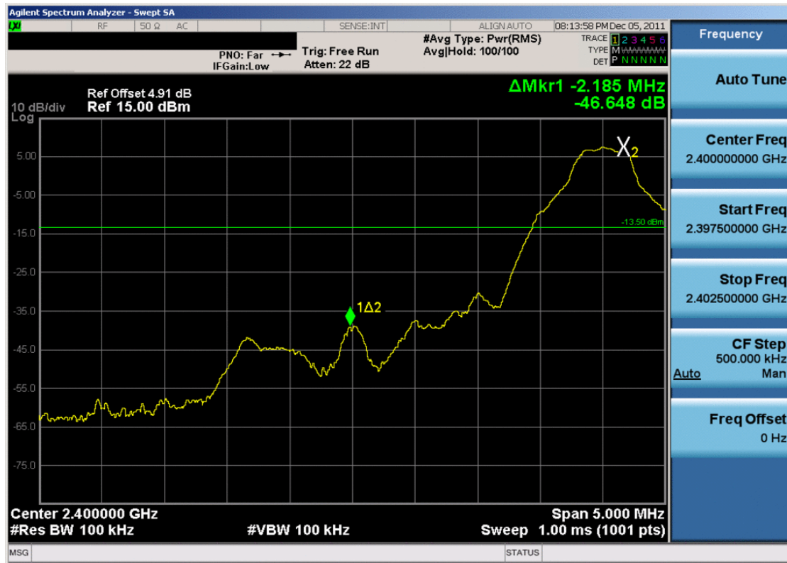
Plot 6-10. Band Edge Plot (Bluetooth, 1Mbps – Ch. 0)
