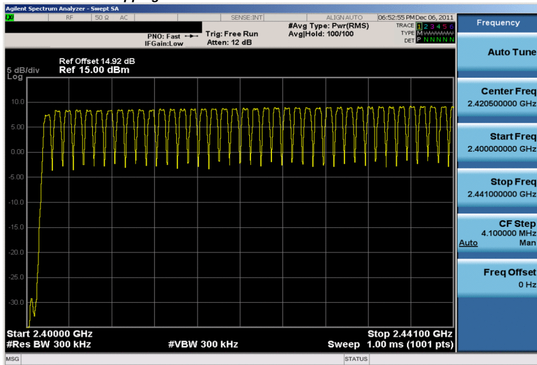
Plot 6-14. Low End Spectrum Channel Hopping Plot (Bluetooth)
