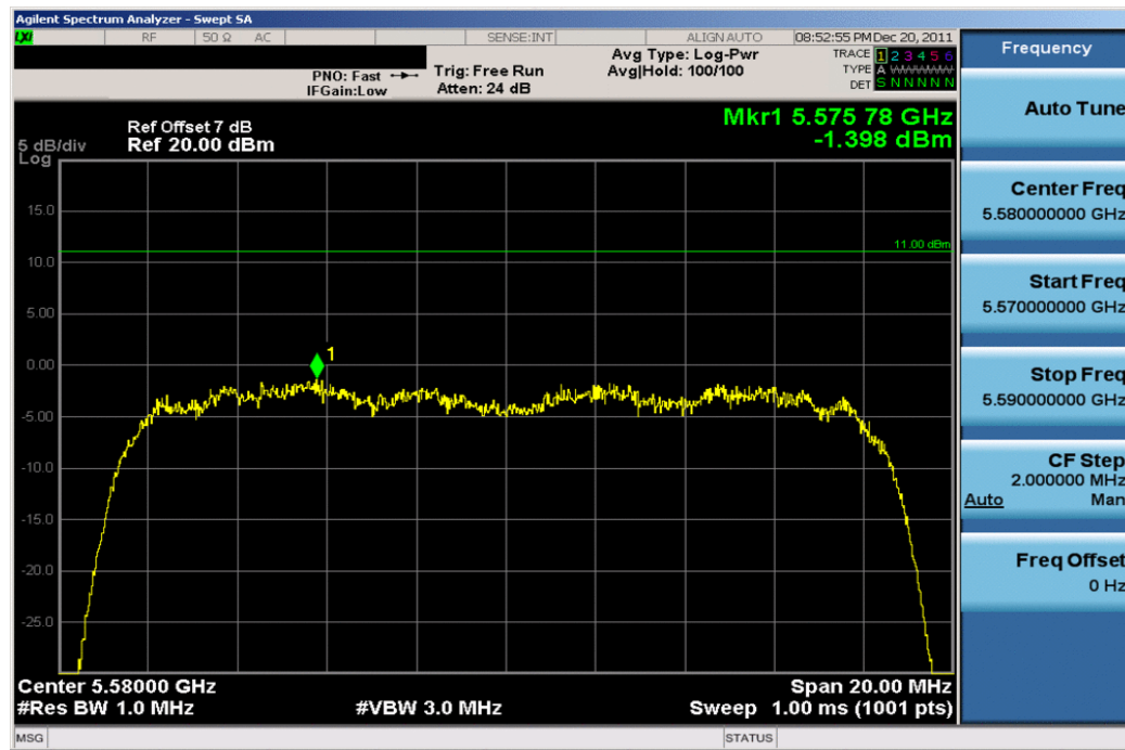
Plot 6-32. Peak Power Spectral Density Plot (802.11a (UNII Band 3) – Ch. 116)
