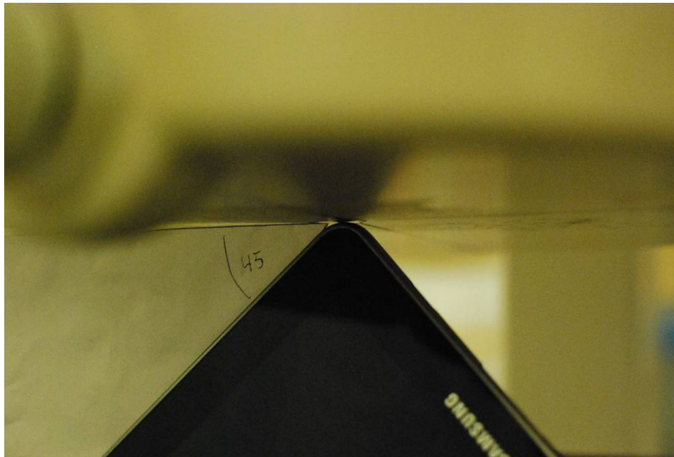
SAR Test Setup Photo 12 - 45° Vertex at 0.0 cm
