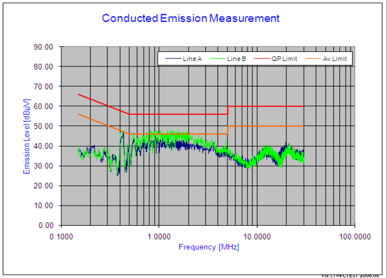
Plot 6-53. Line Conducted Plot with 802.11b
