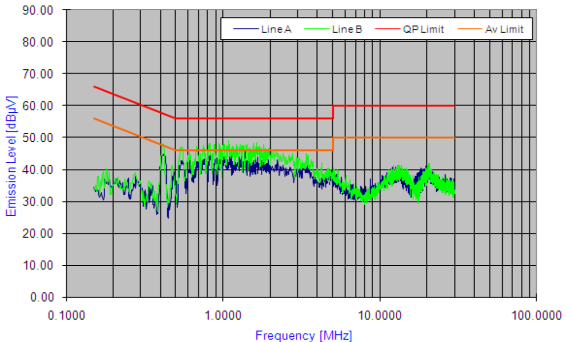
Plot 6-55. Line Conducted Plot with 802.11n (2.4GHz)
