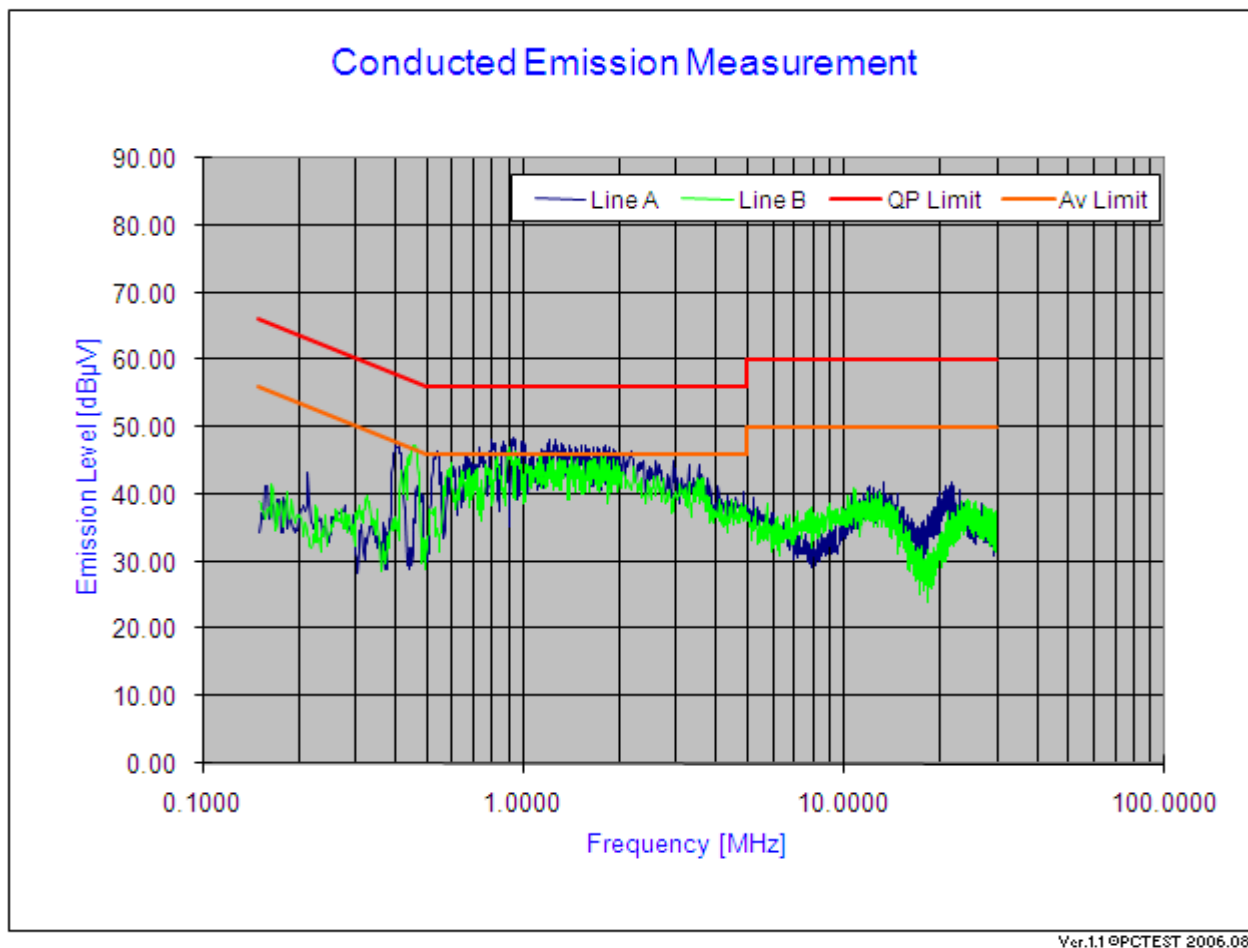
Plot 6-22. Line Conducted Plot with Bluetooth
