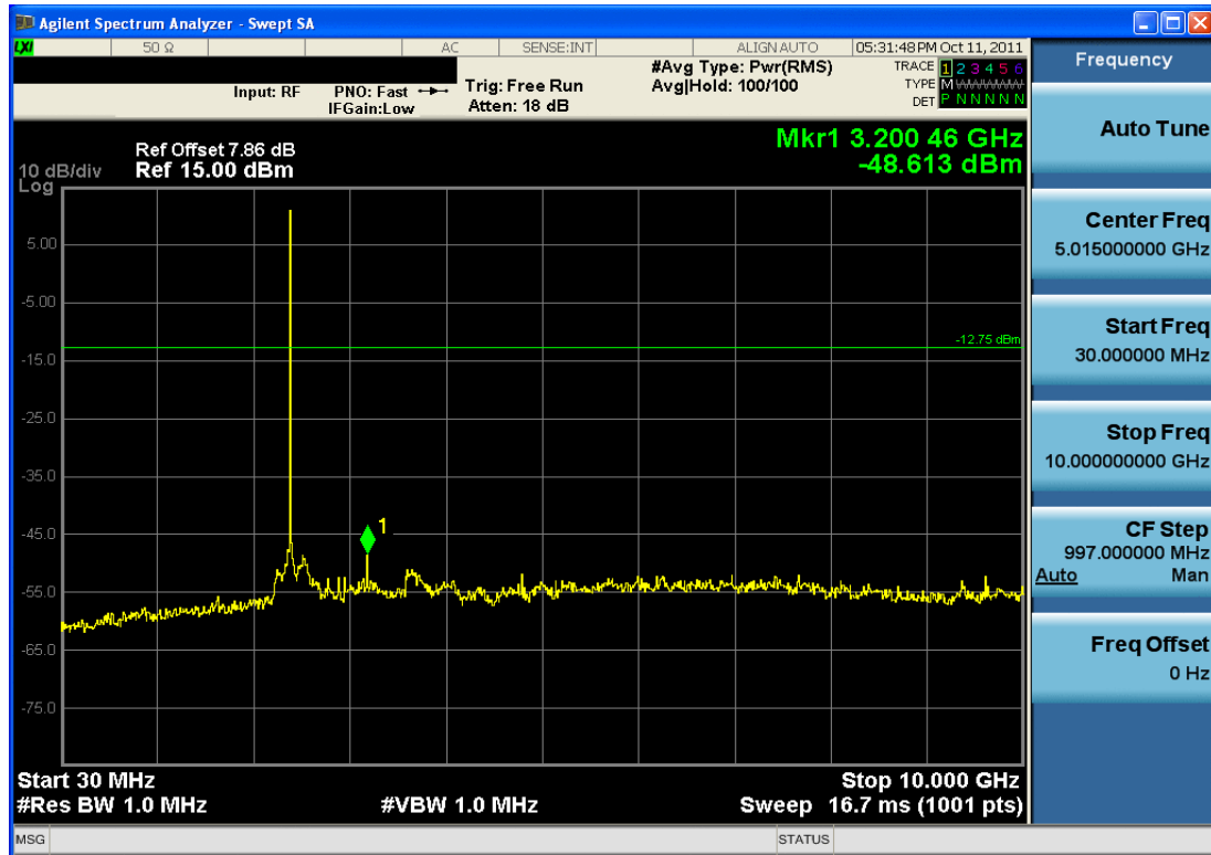
Plot 6-16. Conducted Spurious Plot (Bluetooth, 2Mbps – Ch. 0)
