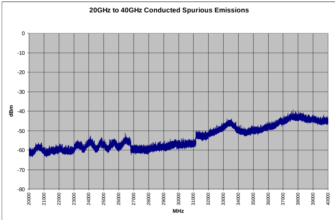
Plot 6-50. Conducted Spurious Plot (802.11a – Ch. 157)
