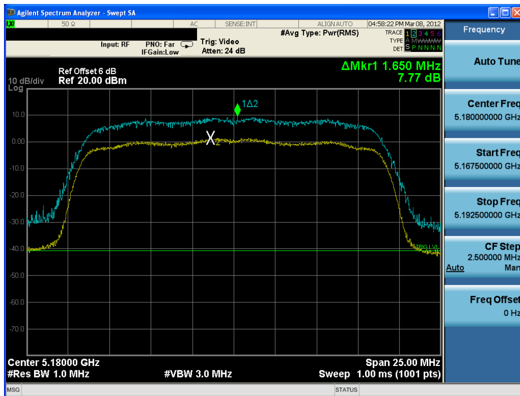
Plot 6-40. Peak Excursion Ratio Plot (802.11n (UNII Band 1) – Ch. 36)
