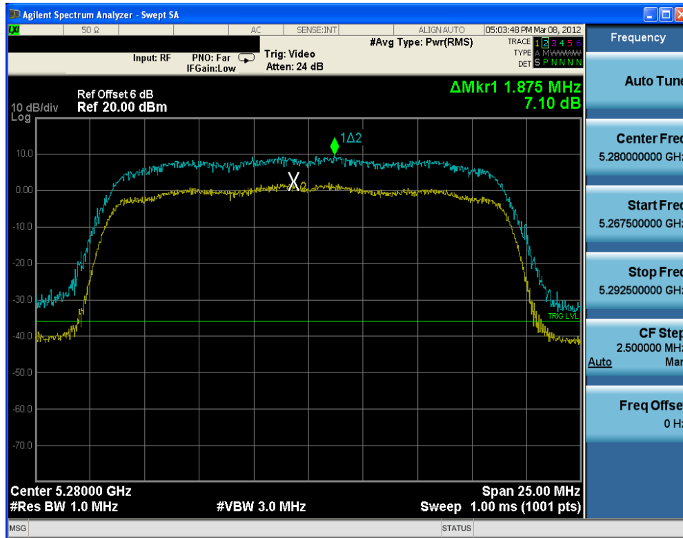
Plot 6-47. Peak Excursion Ratio Plot (802.11n (UNII Band 2) – Ch. 56)
