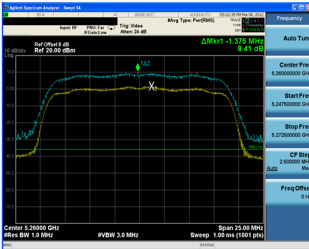
Plot 6-46. Peak Excursion Ratio Plot (802.11n (UNII Band 2) – Ch. 52)
