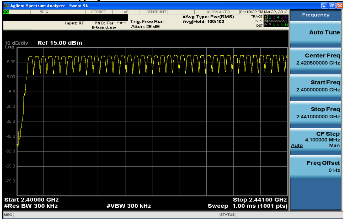
Plot 6-16. Low End Spectrum Channel Hopping Plot (Bluetooth)
