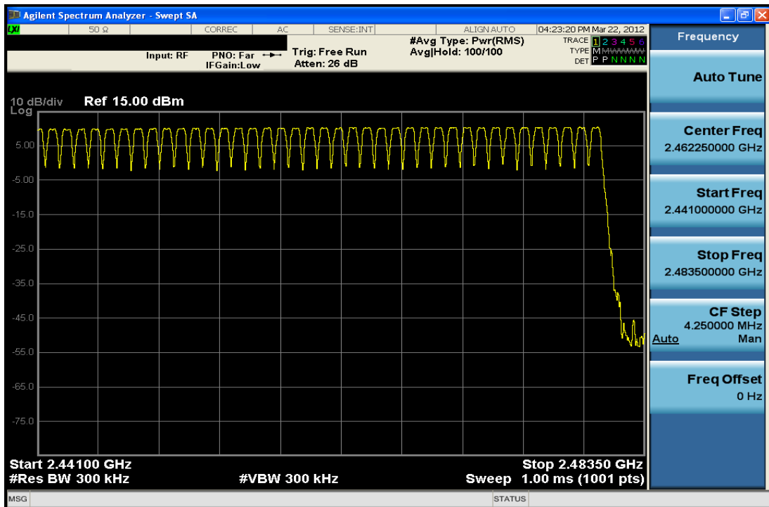
Plot 6-17. High End Spectrum Channel Hopping Plot (Bluetooth)
