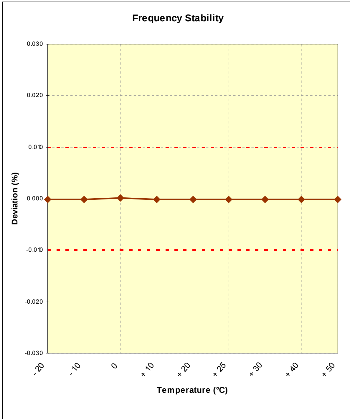
Figure 8-3. Frequency Stability Plot
