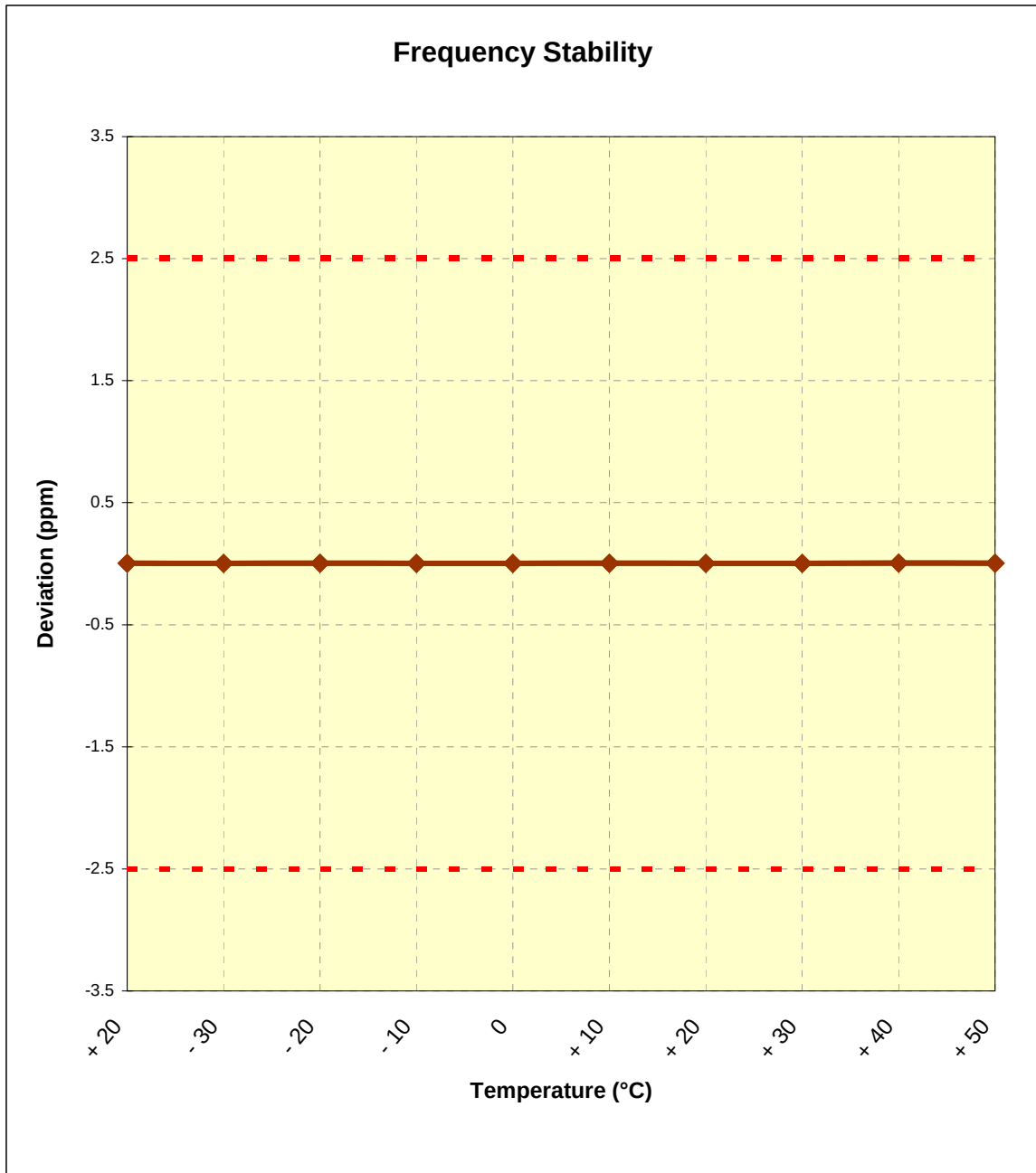
Plot 6-1. Frequency Stability Graph (PCS GSM Mode – Ch. 661)
