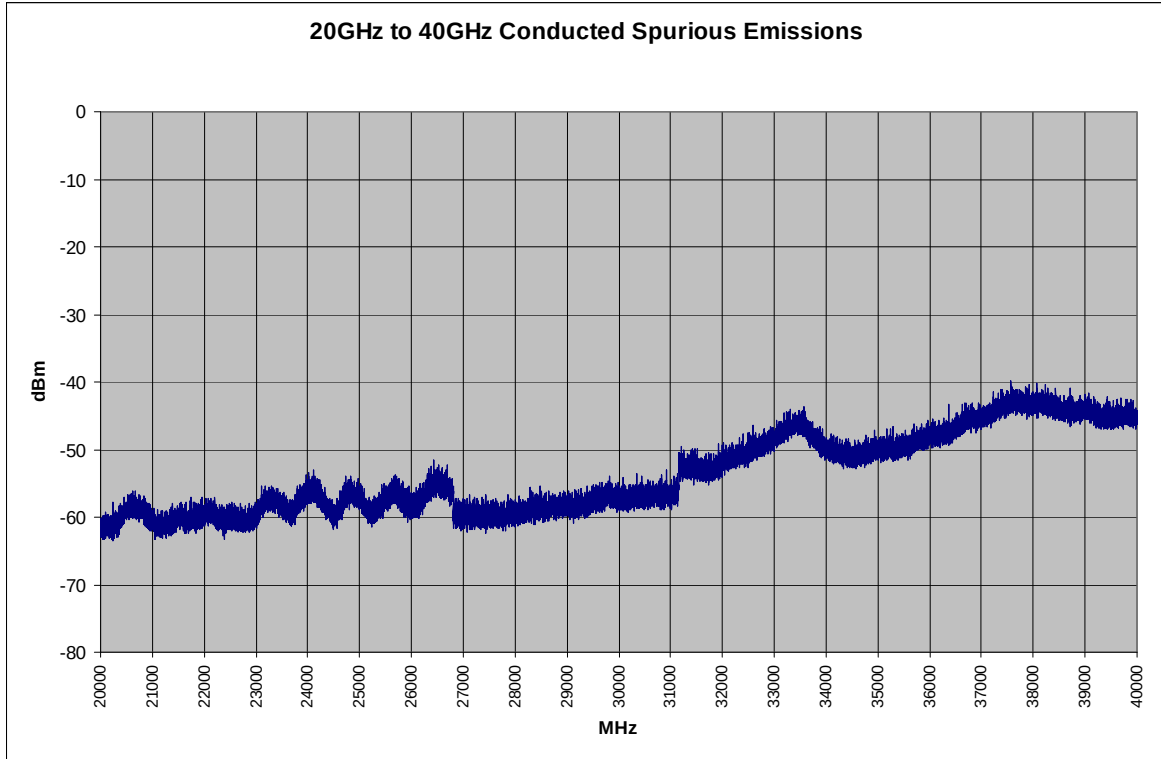
Plot 6-48. Conducted Spurious Plot (802.11a – Ch. 149)
