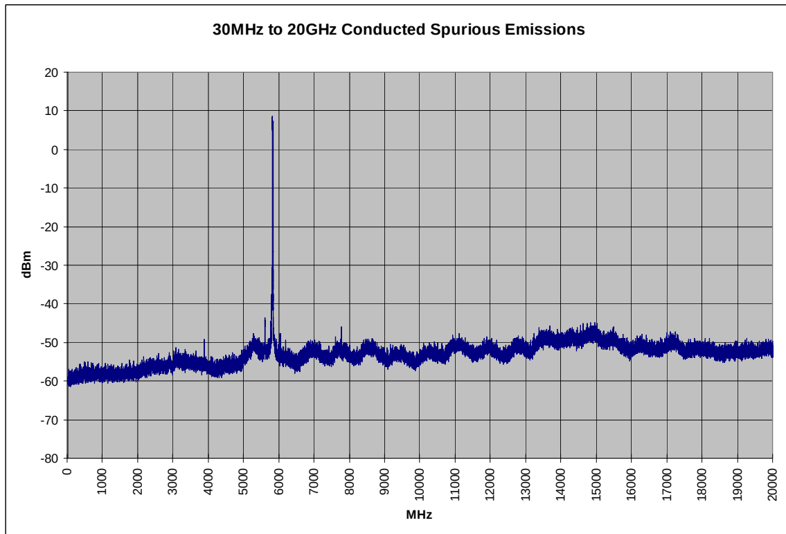
Plot 6-51. Conducted Spurious Plot (802.11a – Ch. 165)
