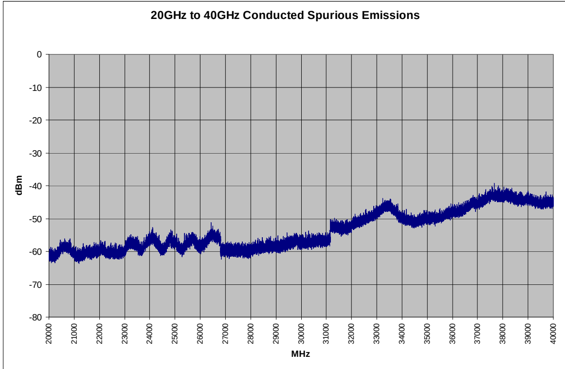
Plot 6-50. Conducted Spurious Plot (802.11a – Ch. 157)
