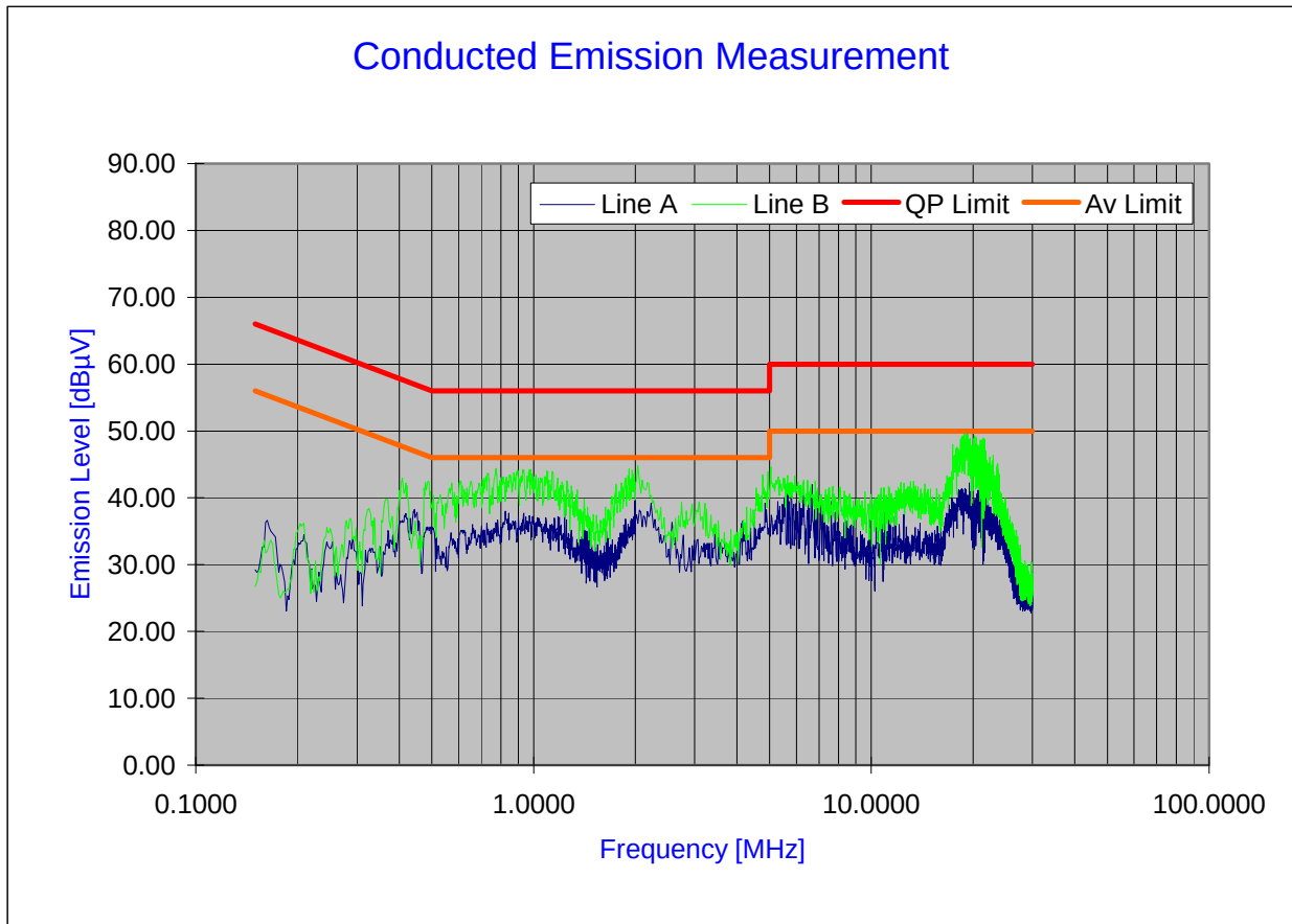
Plot 6-54. Line Conducted Plot with 802.11a
