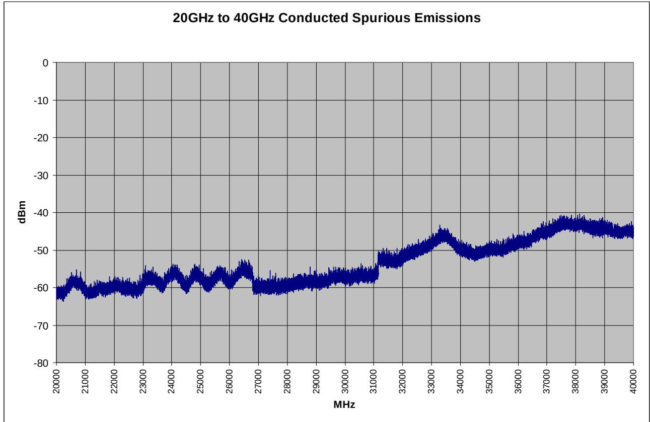
Plot 6-52. Conducted Spurious Plot (802.11a – Ch. 165)
