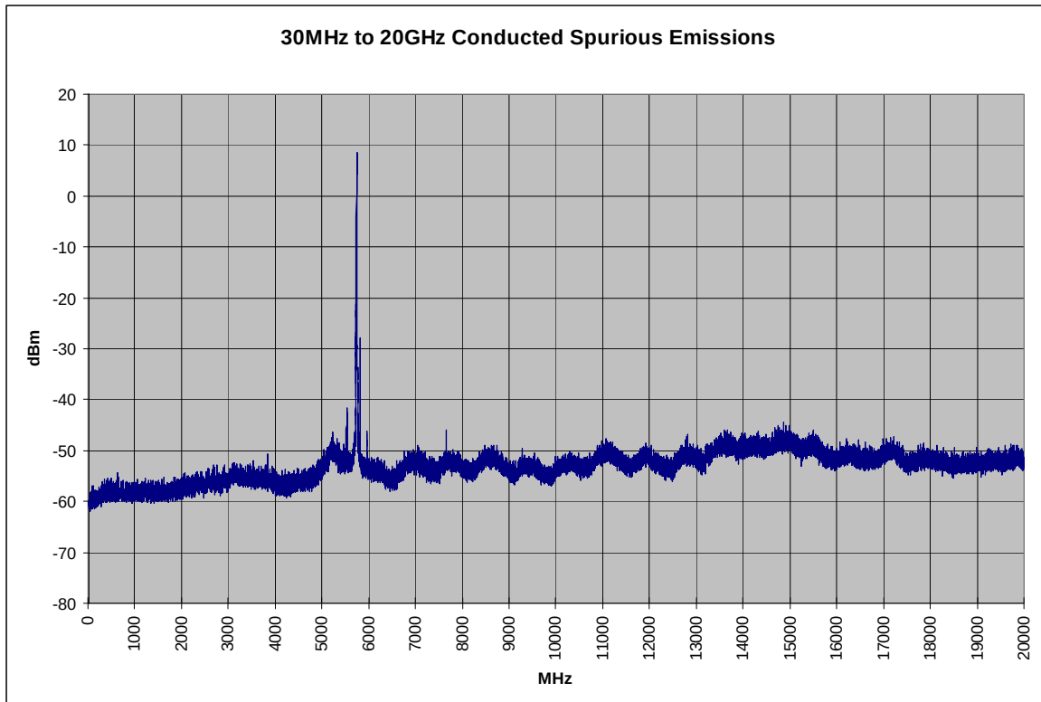
Plot 6-47. Conducted Spurious Plot (802.11a – Ch. 149)
