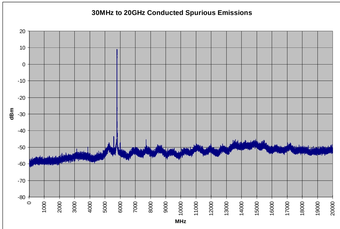
Plot 6-49. Conducted Spurious Plot (802.11a – Ch. 157)
