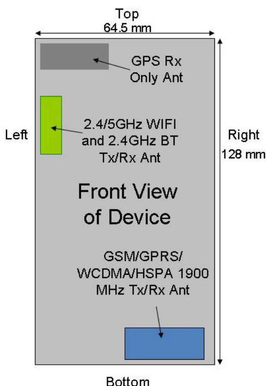
Figure 1-2 DUT Antenna Locations
