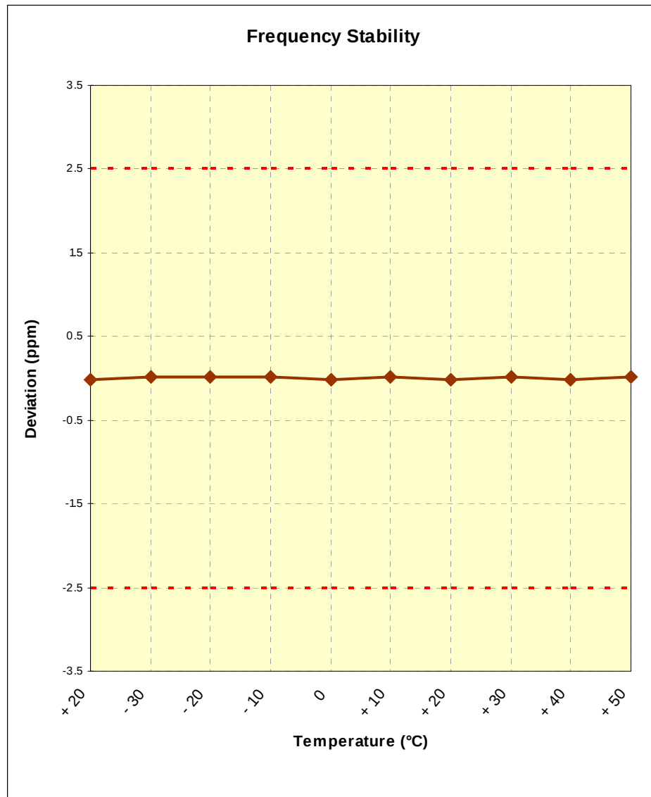
Figure 6-1. Frequency Stability Graph (PCS GSM Mode – Ch. 661)
