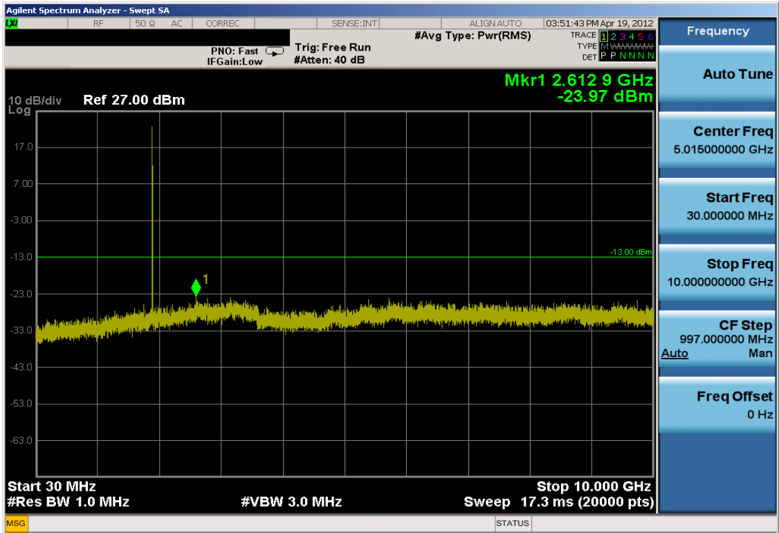
Plot 7-19. Conducted Spurious Plot (PCS WCDMA Mode – Ch. 9538)
