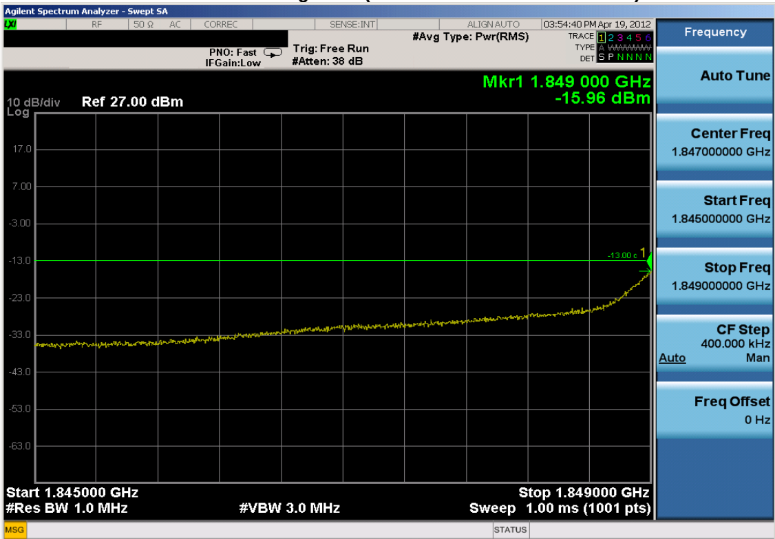
Plot 7-14. 4MHz Span Plot (PCS WCDMA Mode – Ch. 9262)
