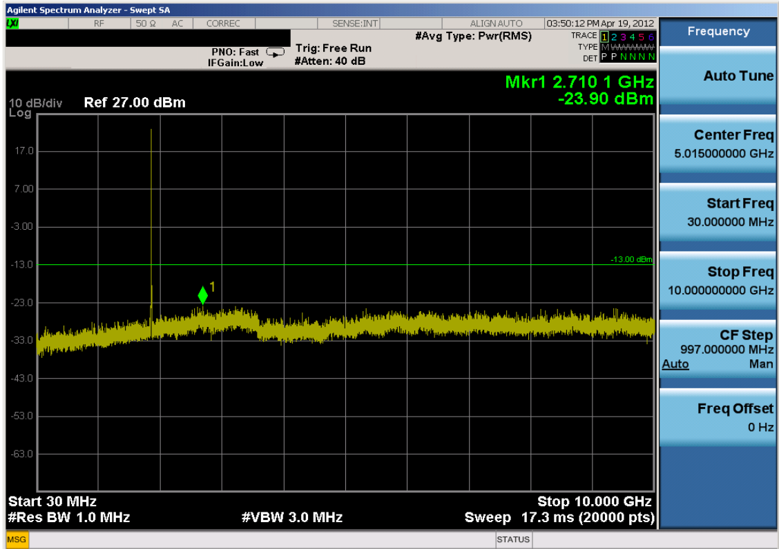
Plot 7-15. Conducted Spurious Plot (PCS WCDMA Mode – Ch. 9400)
