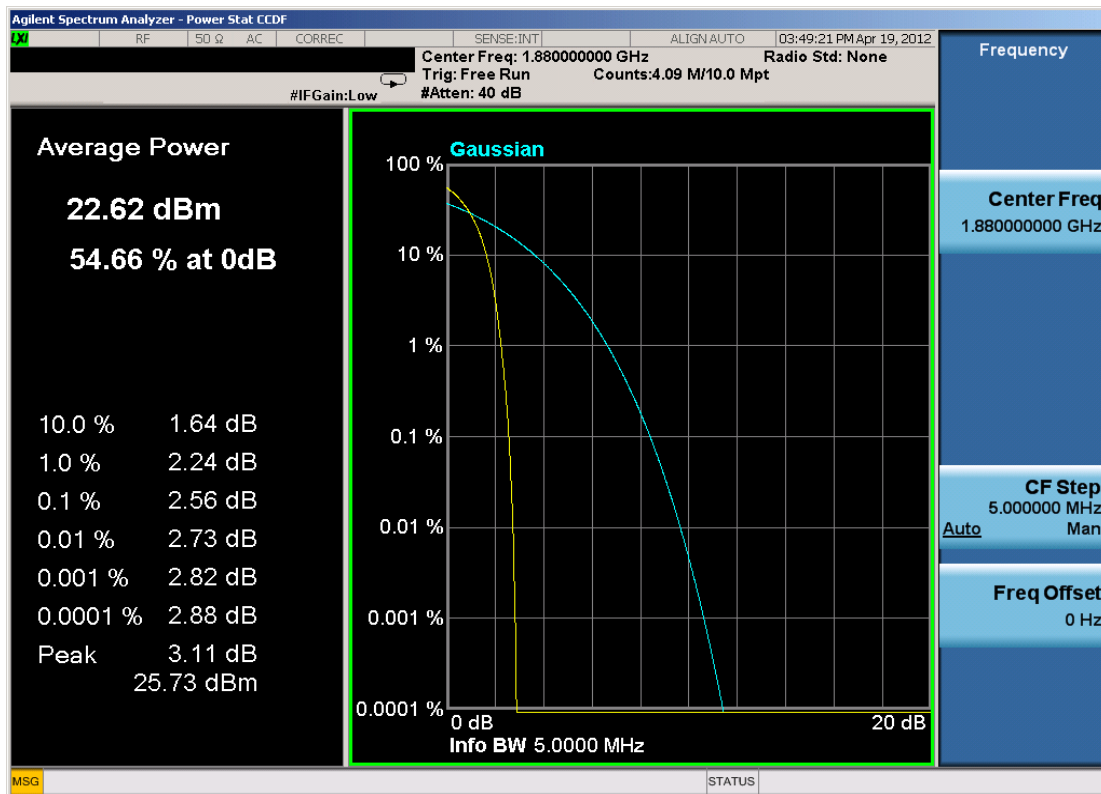
Plot 7-18. Peak-Average Ratio Plot (PCS WCDMA Mode – Ch. 9400)
