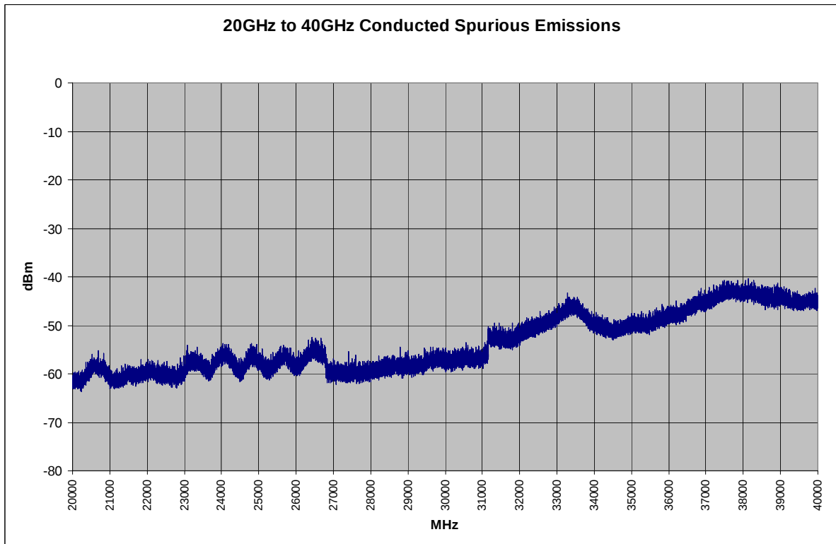
Plot 6-52. Conducted Spurious Plot (802.11a – Ch. 165)
