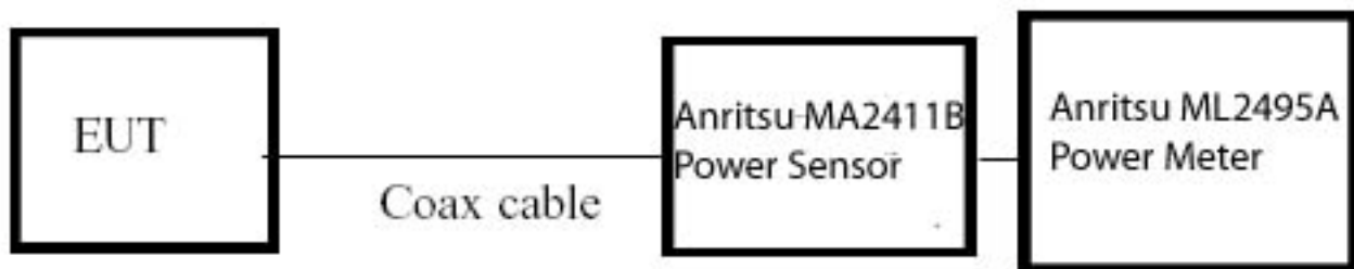
Figure 6-3. Test Instrument & Measurement Setup
