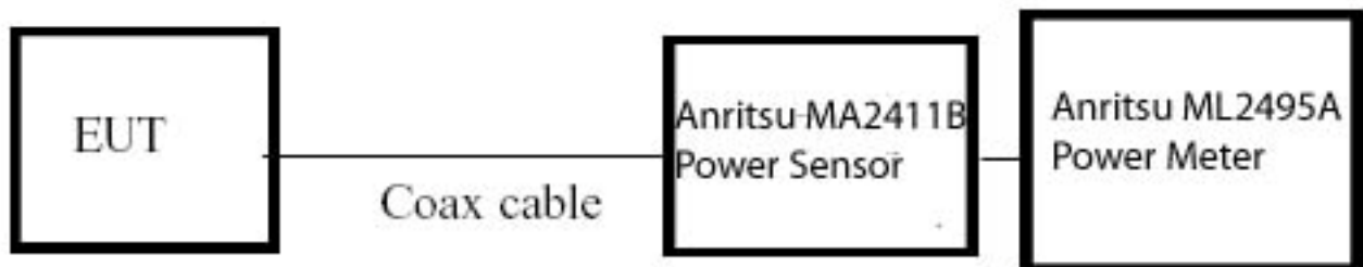
Figure 6-2. Test Instrument & Measurement Setup
