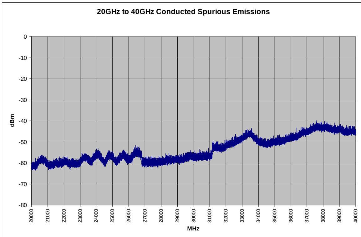
Plot 6-48. Conducted Spurious Plot (802.11a – Ch. 149)
