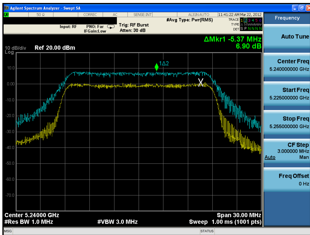
Plot 6-42. Peak Excursion Ratio Plot (802.11n (UNII Band 1) – Ch. 48)
