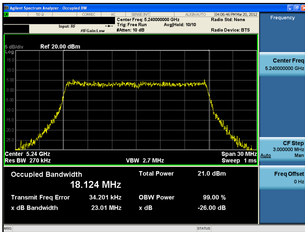
Plot 6-6. 26dB Bandwidth Plot (802.11n (UNII Band 1) – Ch. 48)
