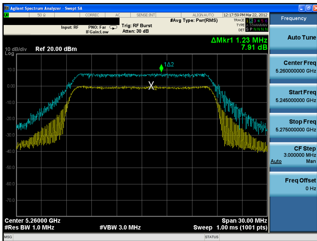
Plot 6-46. Peak Excursion Ratio Plot (802.11n (UNII Band 2) – Ch. 52)
