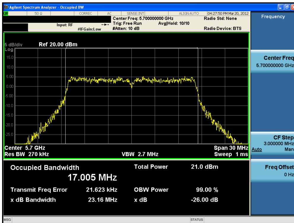
Plot 6-15. 26dB Bandwidth Plot (802.11a (UNII Band 3) – Ch. 140)
