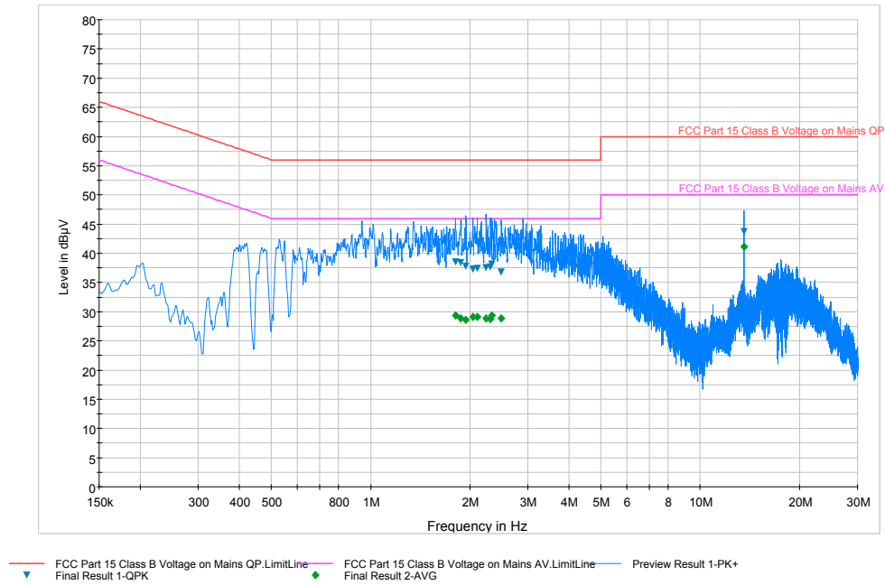
Plot 8-1. Line-Conducted Test Plot (L1)
