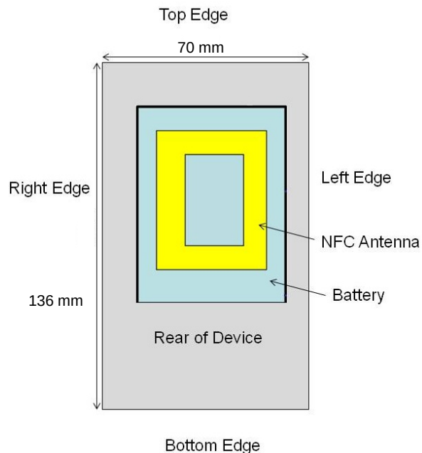
Figure 1-1 NFC Antenna Location on the Battery
