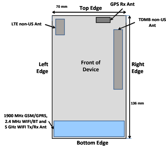
Figure 1-2 DUT Antenna Locations
