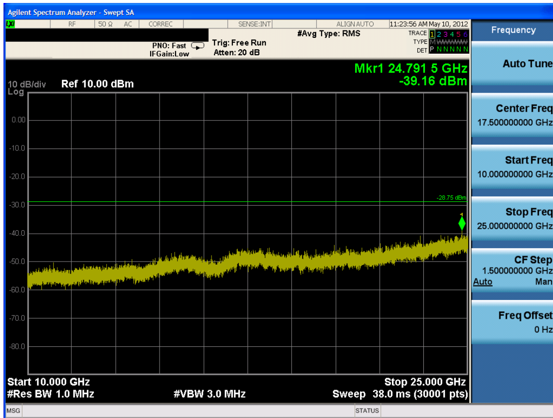
Plot 6-14. Conducted Spurious Plot (Bluetooth (LE) – Ch. 39)
