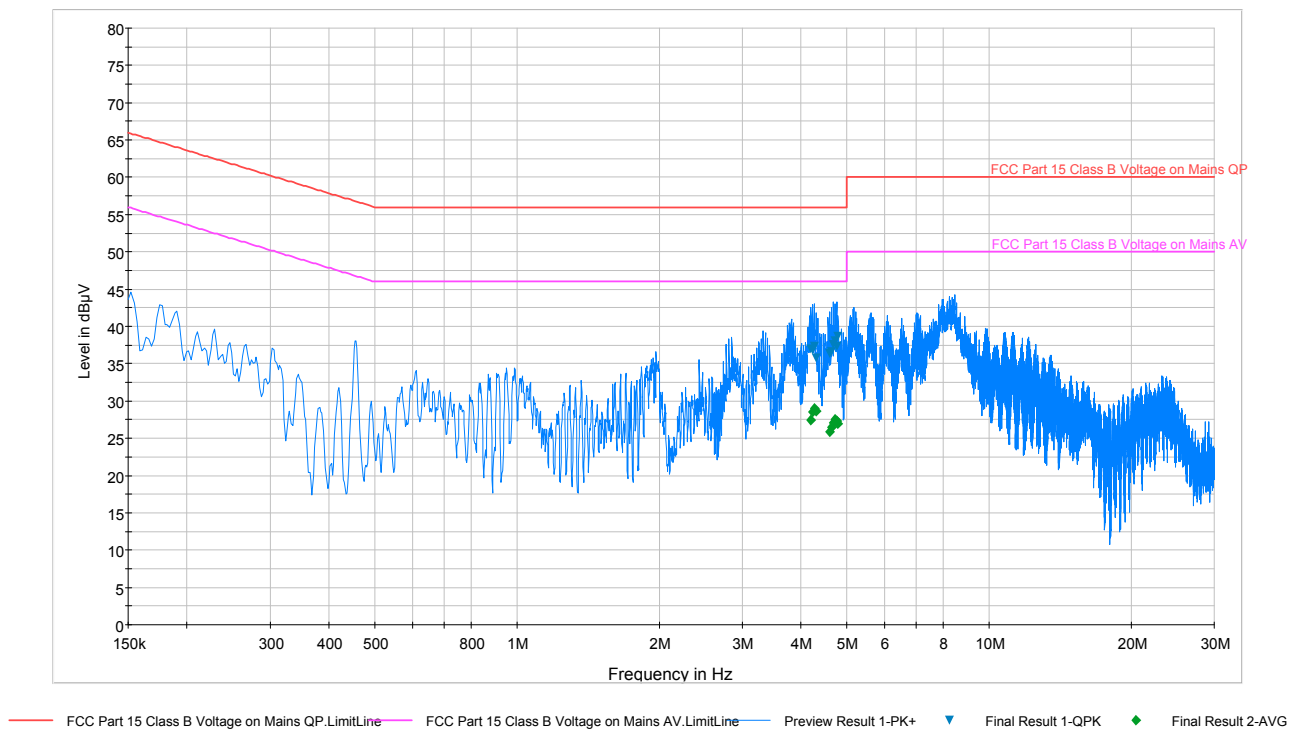
Plot 6-15. Line Conducted Plot with Bluetooth (LE) – Line 1
