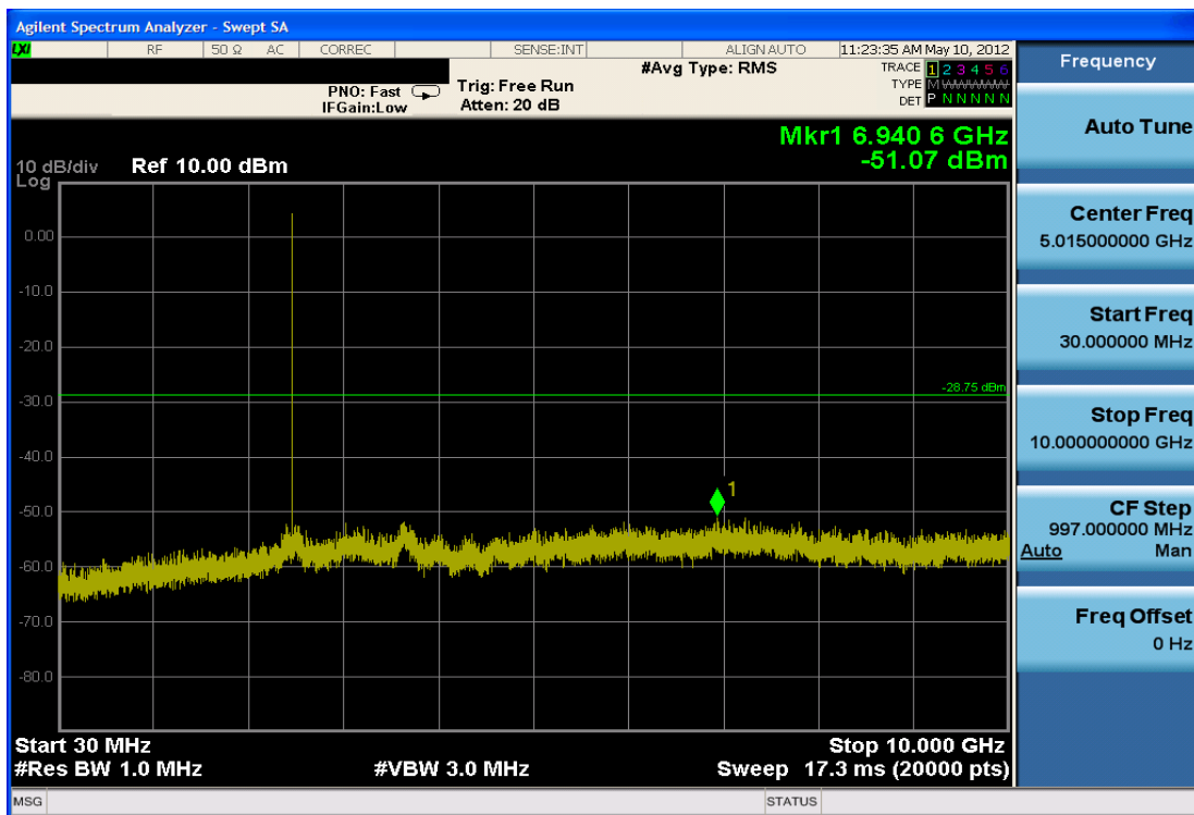
Plot 6-13. Conducted Spurious Plot (Bluetooth (LE) – Ch. 39)
