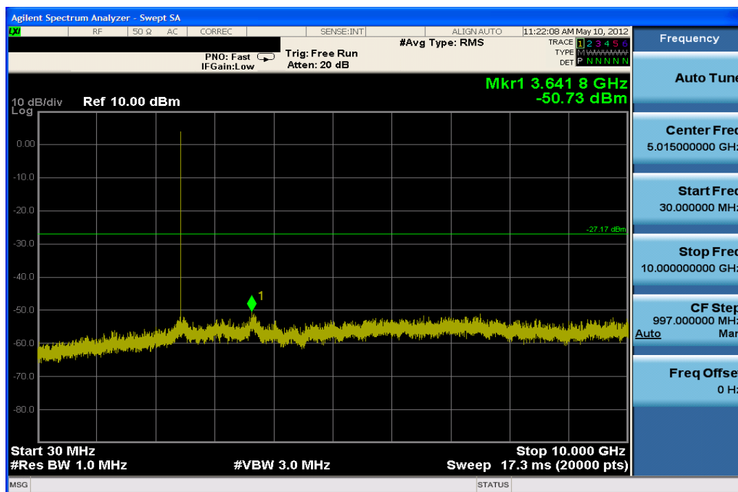
Plot 6-11. Conducted Spurious Plot (Bluetooth (LE) – Ch. 19)
