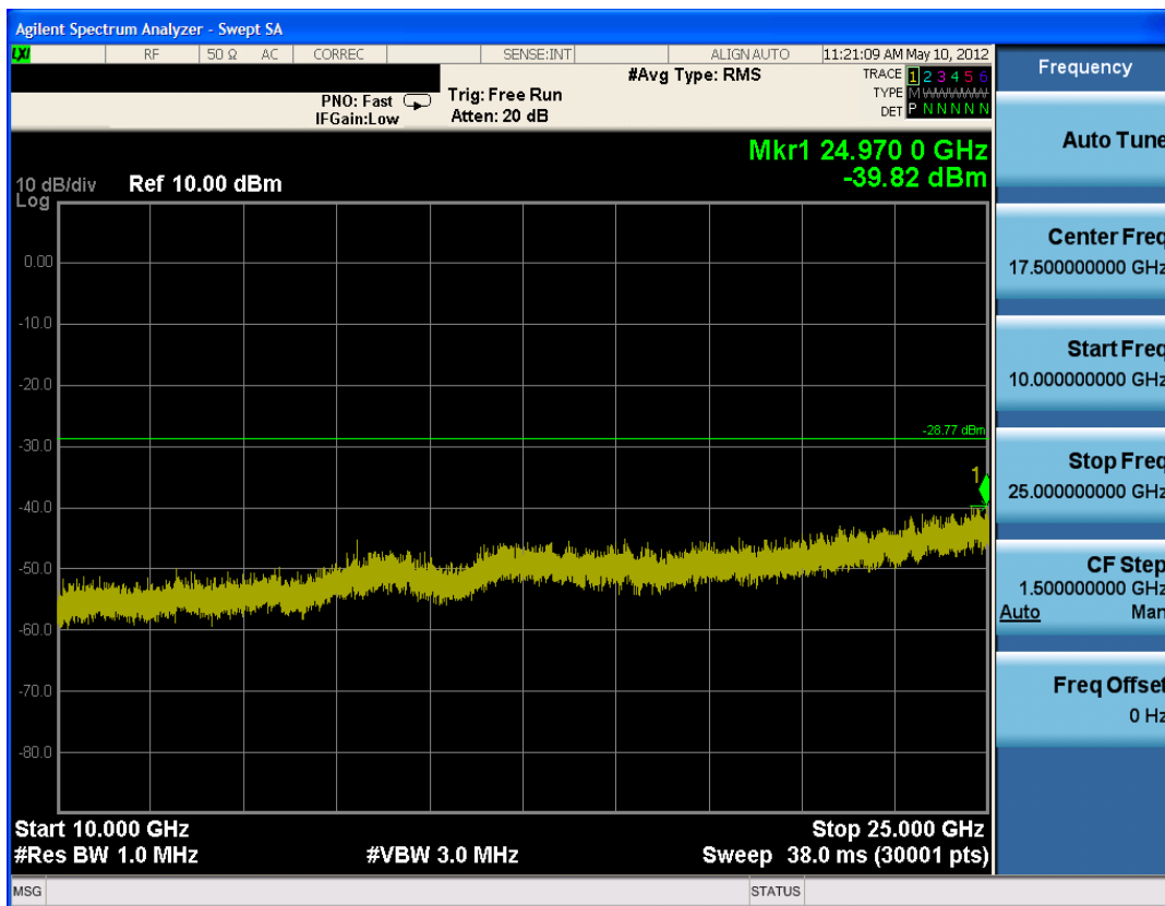
Plot 6-10. Conducted Spurious Plot (Bluetooth (LE) – Ch. 0)
