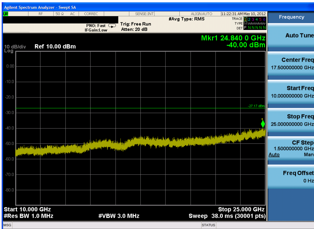
Plot 6-12. Conducted Spurious Plot (Bluetooth (LE) – Ch. 19)
