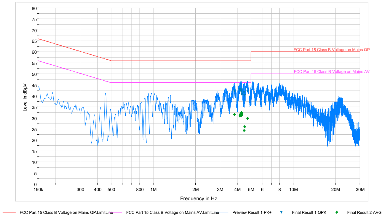
Plot 6-16. Line Conducted Plot with Bluetooth (LE) – Line N
