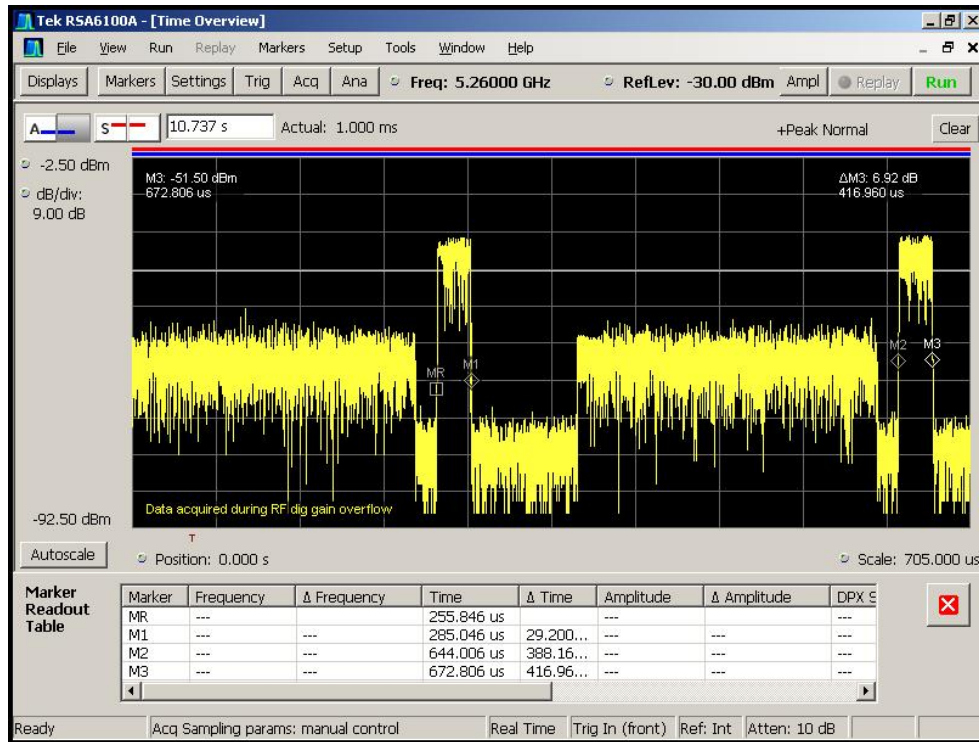
Figure 5-6. Pulse Width After 200ms
