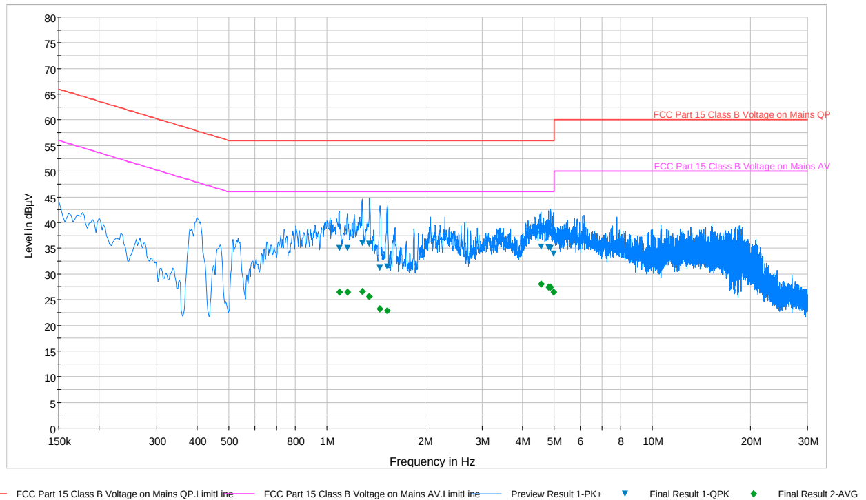
Plot 6-59. Line Conducted Plot with 802.11b – Line 1
