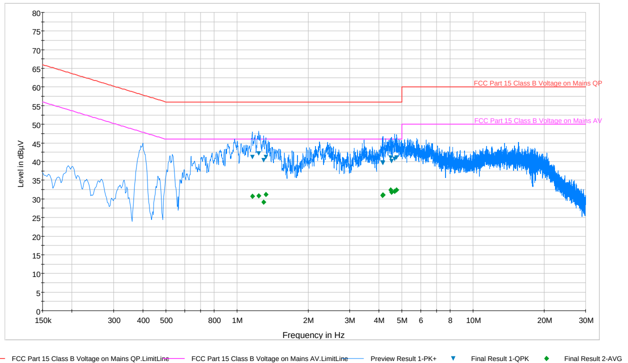
Plot 6-62. Line Conducted Plot with 802.11a – Line N
