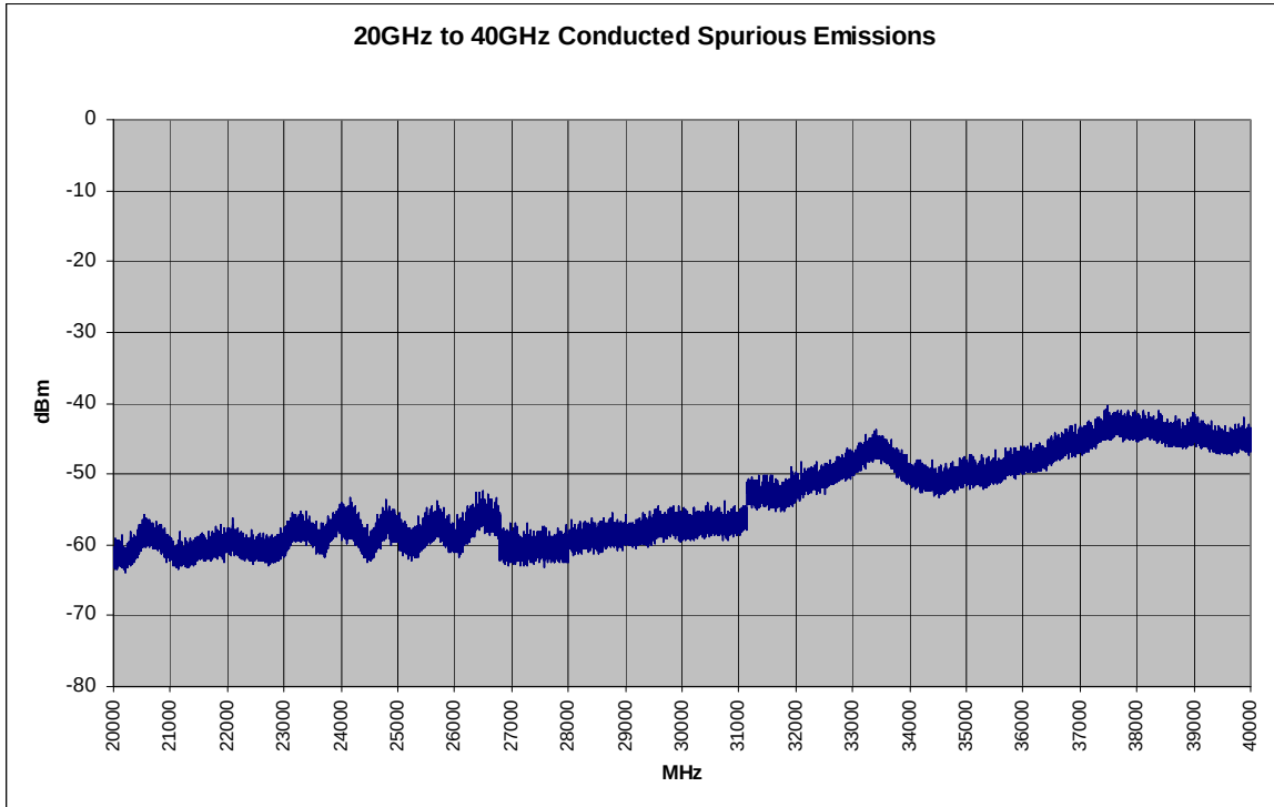
Plot 6-56. Conducted Spurious Plot (802.11a – Ch. 157)
