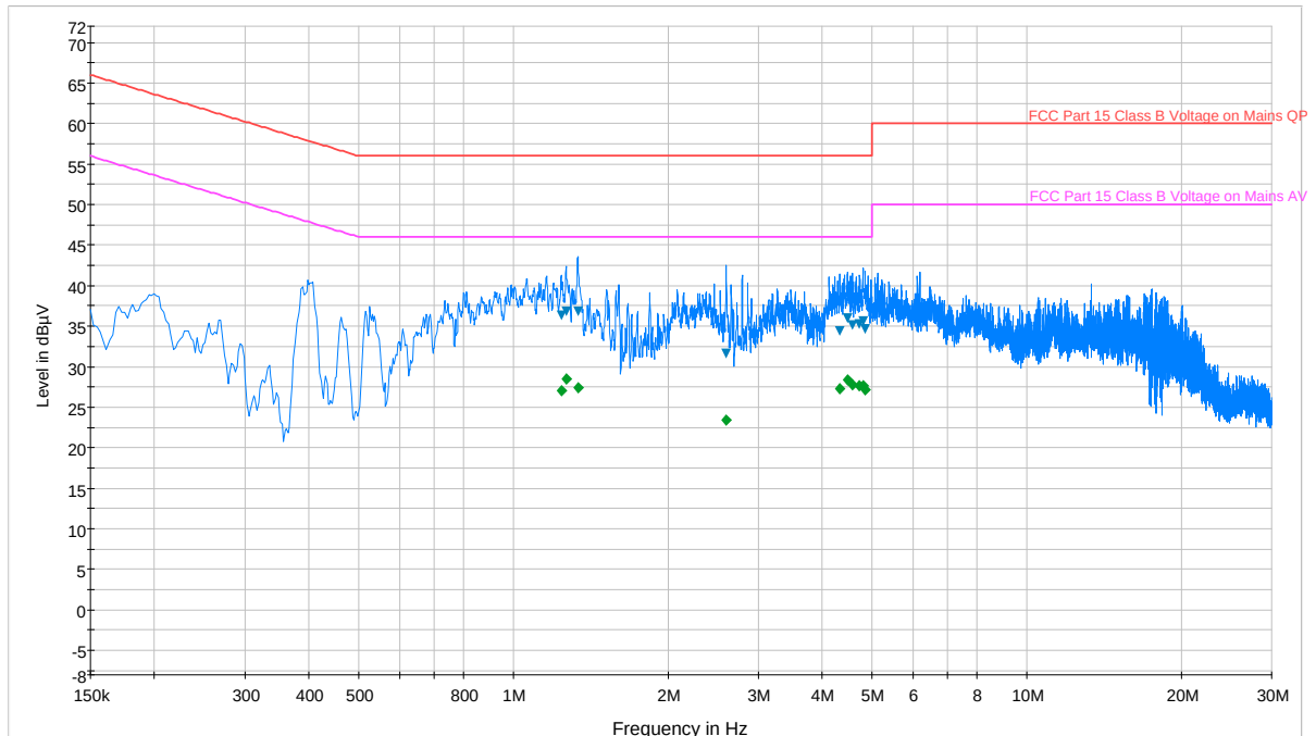
Plot 6-61. Line Conducted Plot with 802.11a – Line 1
