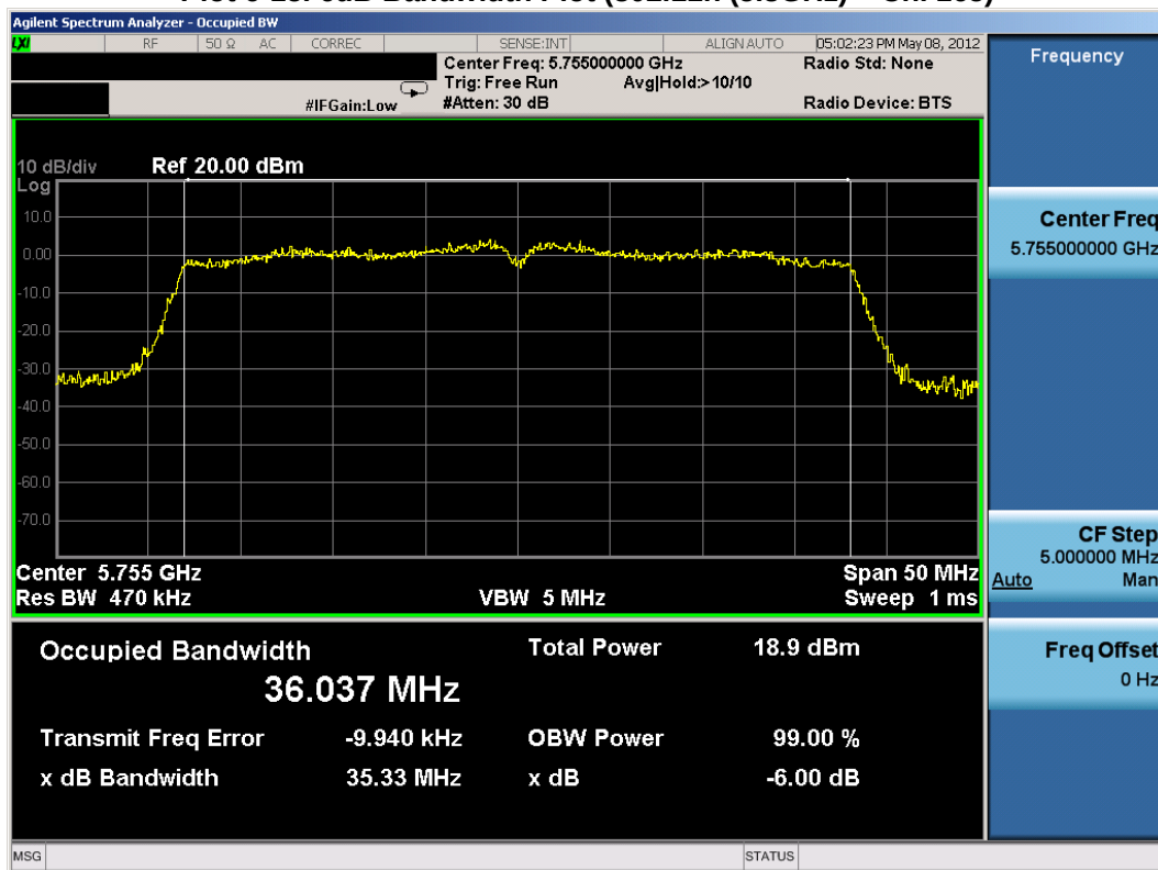
Plot 6-16. 6dB Bandwidth Plot (802.11n (5.8GHz) – Ch. 151) – 40MHz BW
