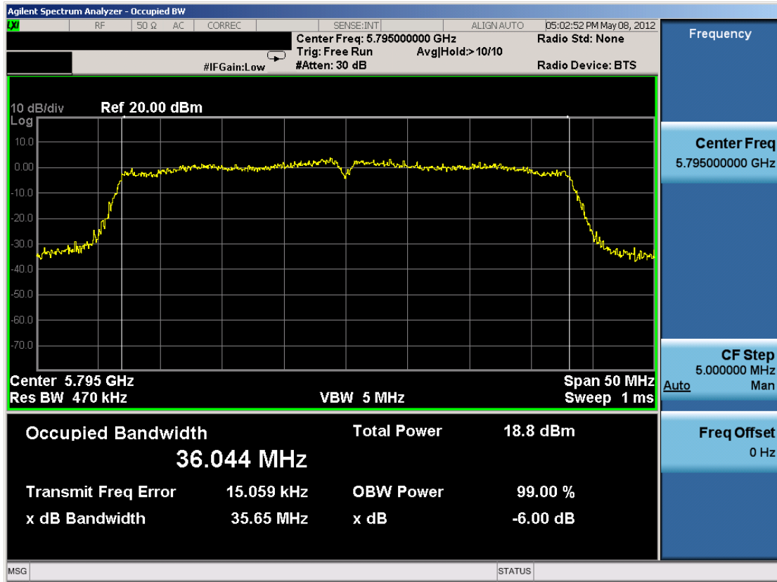
Plot 6-17. 6dB Bandwidth Plot (802.11n (5.8GHz) – Ch. 159) – 40MHz BW
