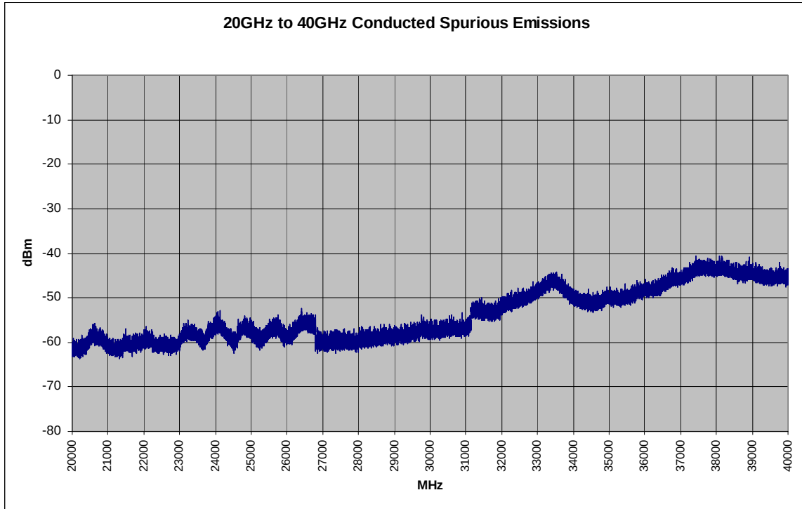
Plot 6-54. Conducted Spurious Plot (802.11a – Ch. 149)
