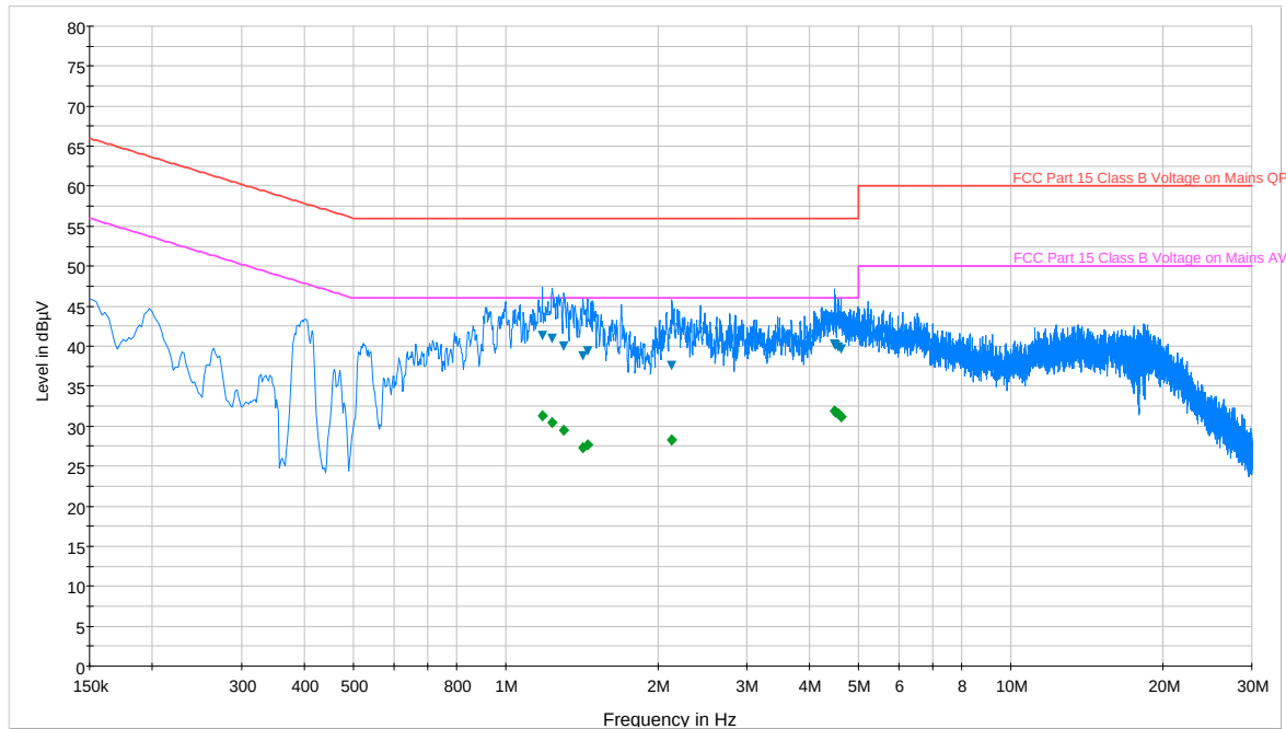
Plot 6-60. Line Conducted Plot with 802.11b – Line N
