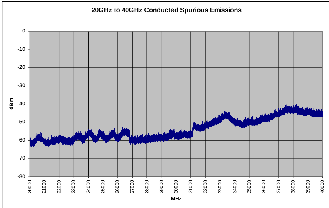
Plot 6-58. Conducted Spurious Plot (802.11a – Ch. 165)
