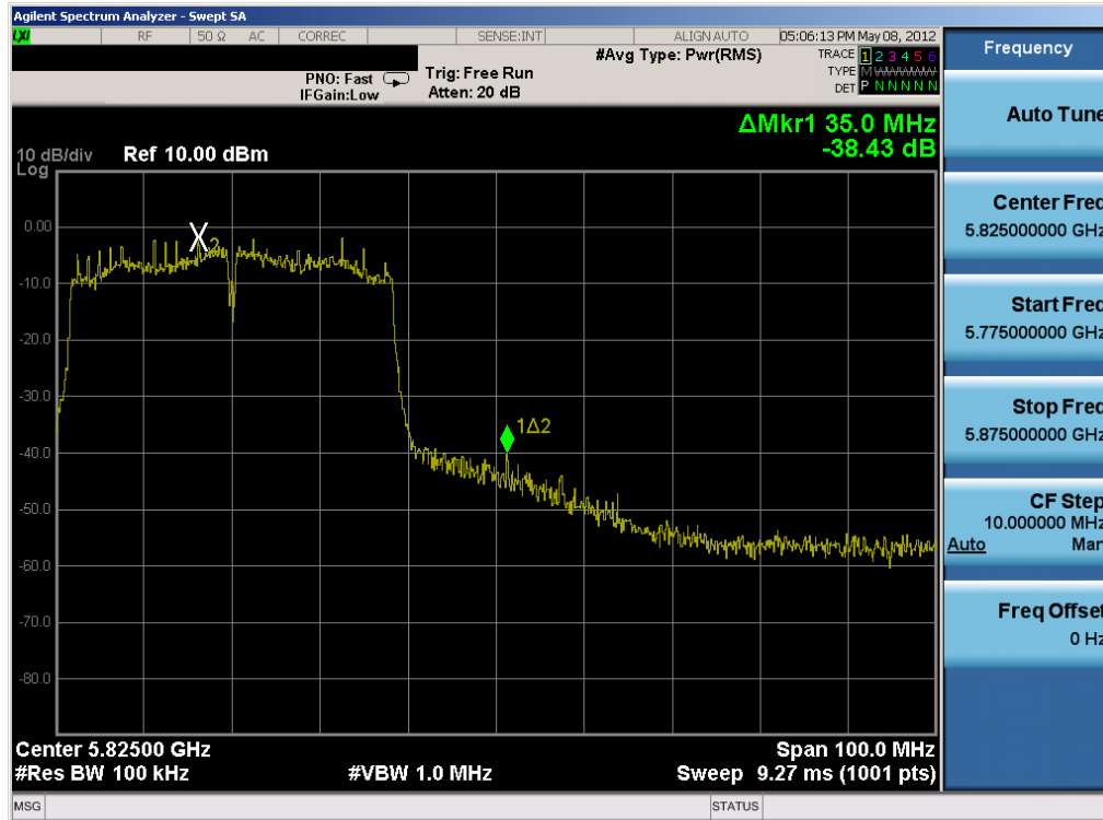
Plot 6-46. Band Edge Plot (802.11n (5.8GHz) – Ch. 159) – 40MHz BW
