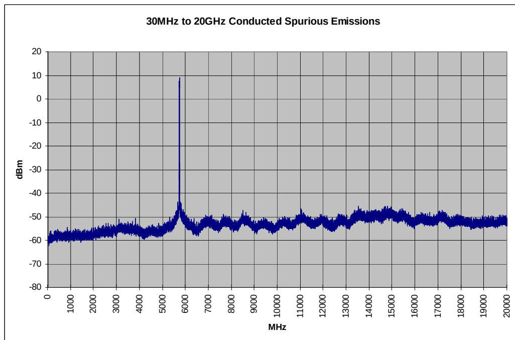
Plot 6-53. Conducted Spurious Plot (802.11a – Ch. 149)
