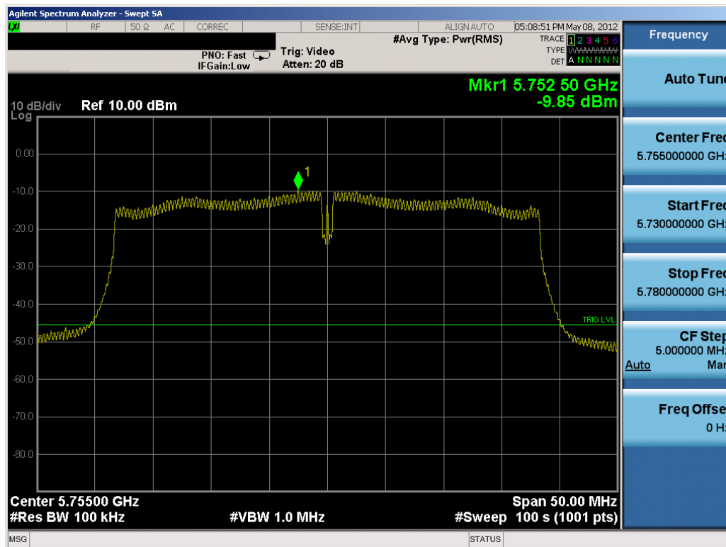
Plot 6-33. Power Spectral Density Plot (802.11n (5.8GHz) – Ch. 151) – 40MHz
