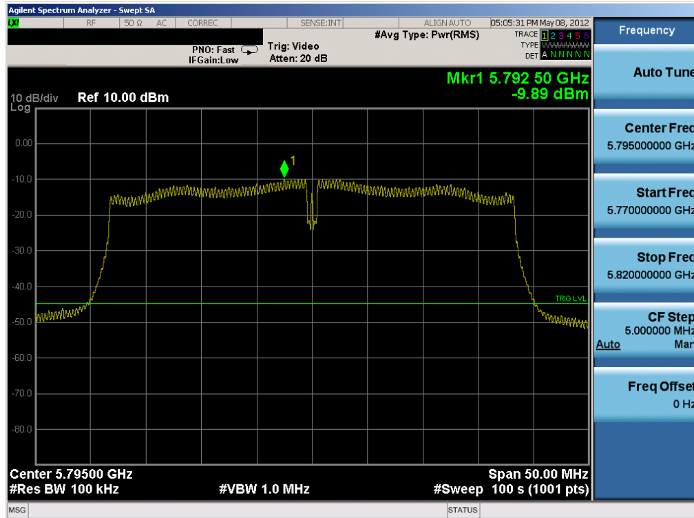
Plot 6-34. Power Spectral Density Plot (802.11n (5.8GHz) – Ch. 159) – 40MHz
