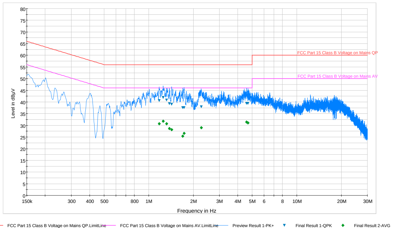
Plot 6-25. Line-Conducted Test Plot (N)
