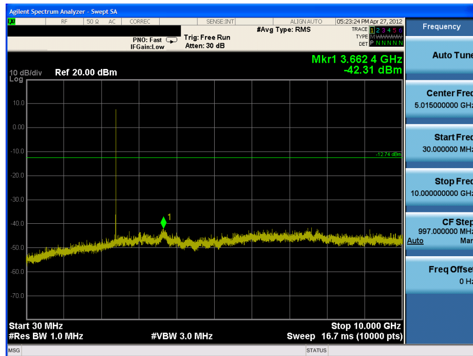
Plot 6-18. Conducted Spurious Plot (Bluetooth, 1Mbps – Ch. 0)
