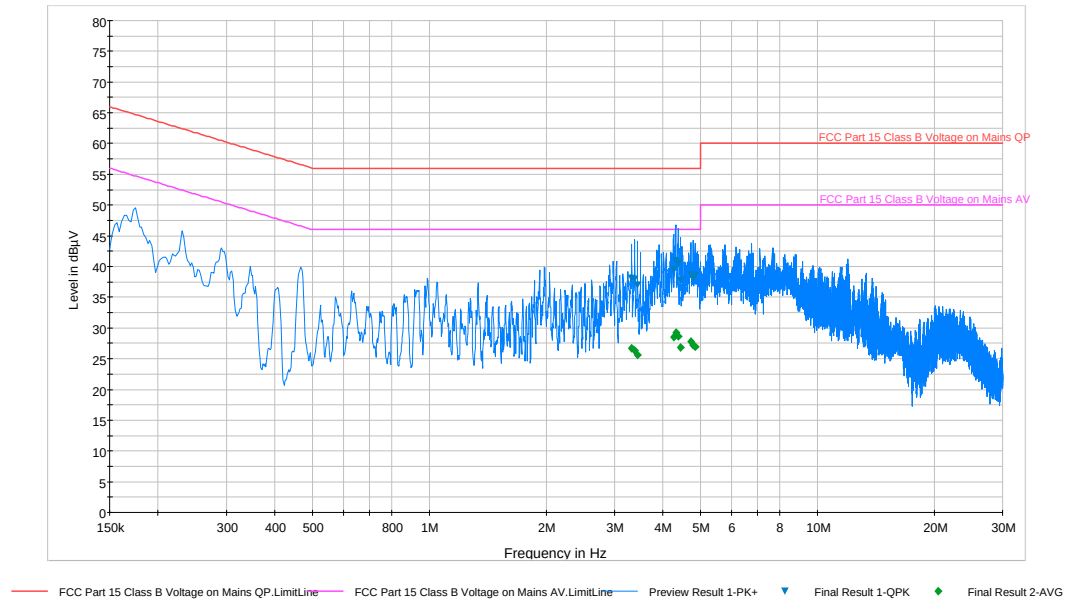
Plot 6-24. Line-Conducted Test Plot (L1)
