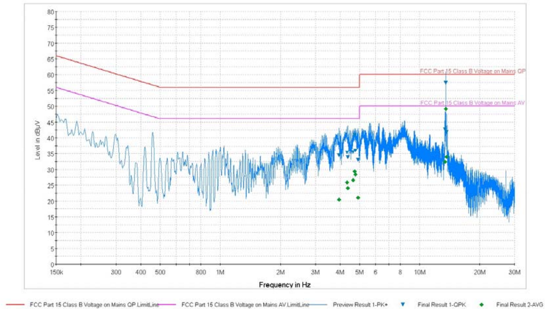
Plot 8-1. Line-Conducted Test Plot (L1)
