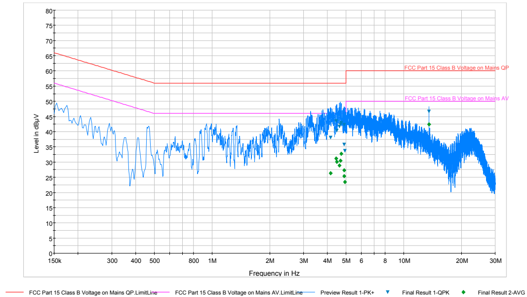
Plot 8-2. Line-Conducted Test Plot (N)
