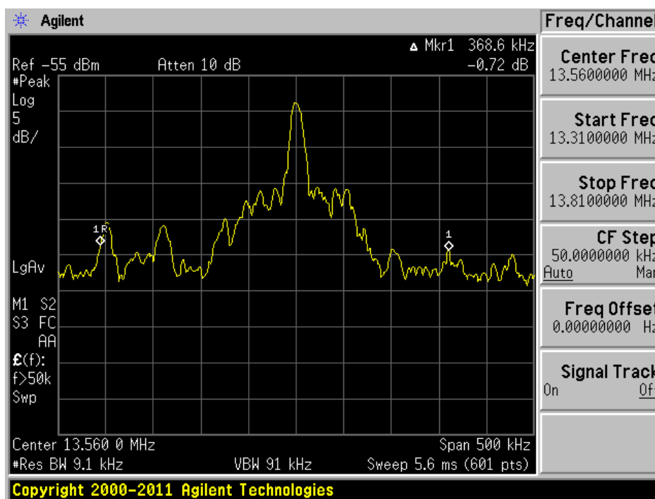
Figure 8-2. 20dB Bandwidth Plot
