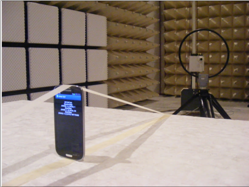
D. Photo of Field Strength & Spurious Emission Test BT LE
