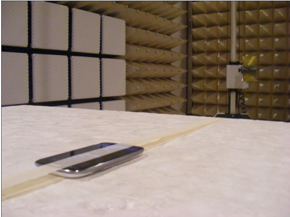
B. Photo of Field Strength & Spurious Emission Test for Bluetooth
