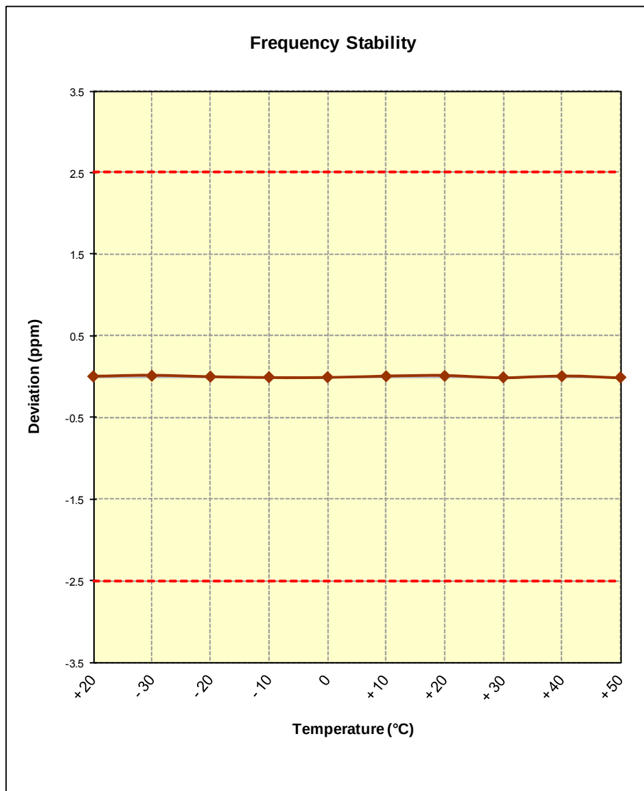
Figure 6-1. Frequency Stability Graph (PCS GSM Mode – Ch. 661)
