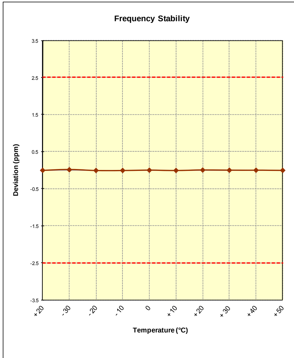
Figure 6-2. Frequency Stability Graph (PCS WCDMA Mode – Ch. 9400)
