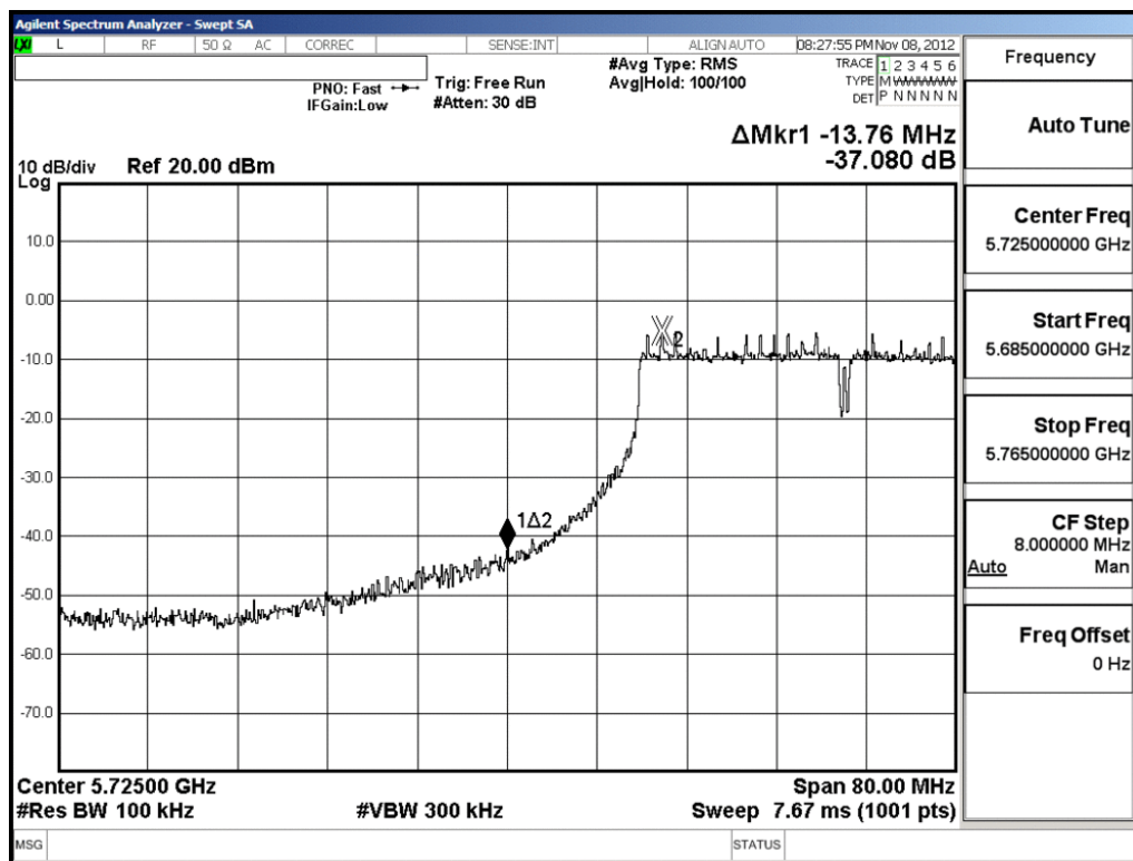
Plot 6-45. Band Edge Plot (40MHz BW 802.11n (5.8GHz) – Ch. 151)
