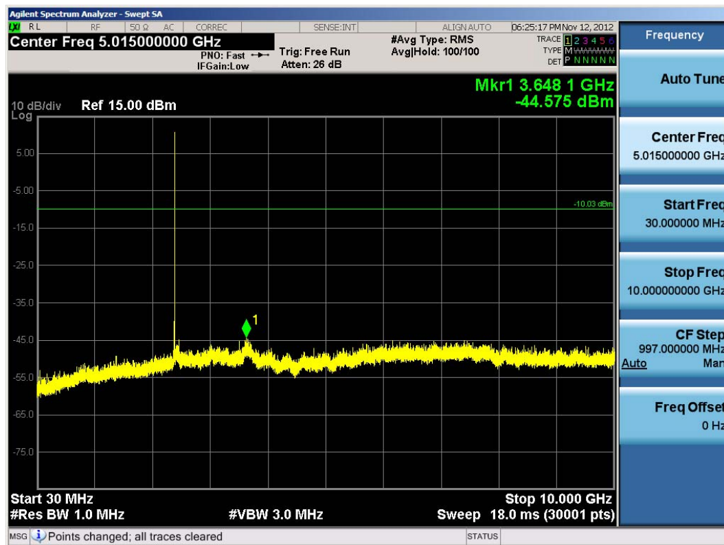
Plot 6-27. Conducted Spurious Plot (Bluetooth, 1Mbps – Ch. 0)
