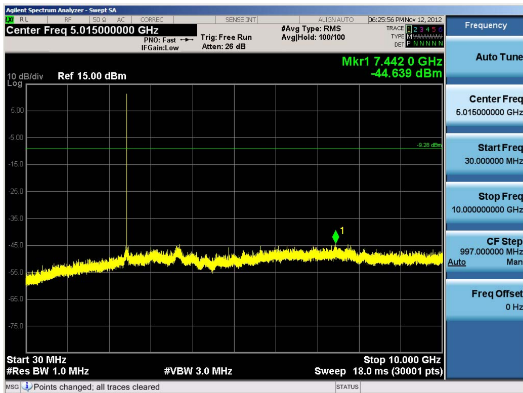
Plot 6-29. Conducted Spurious Plot (Bluetooth, 1Mbps - Ch. 39)
