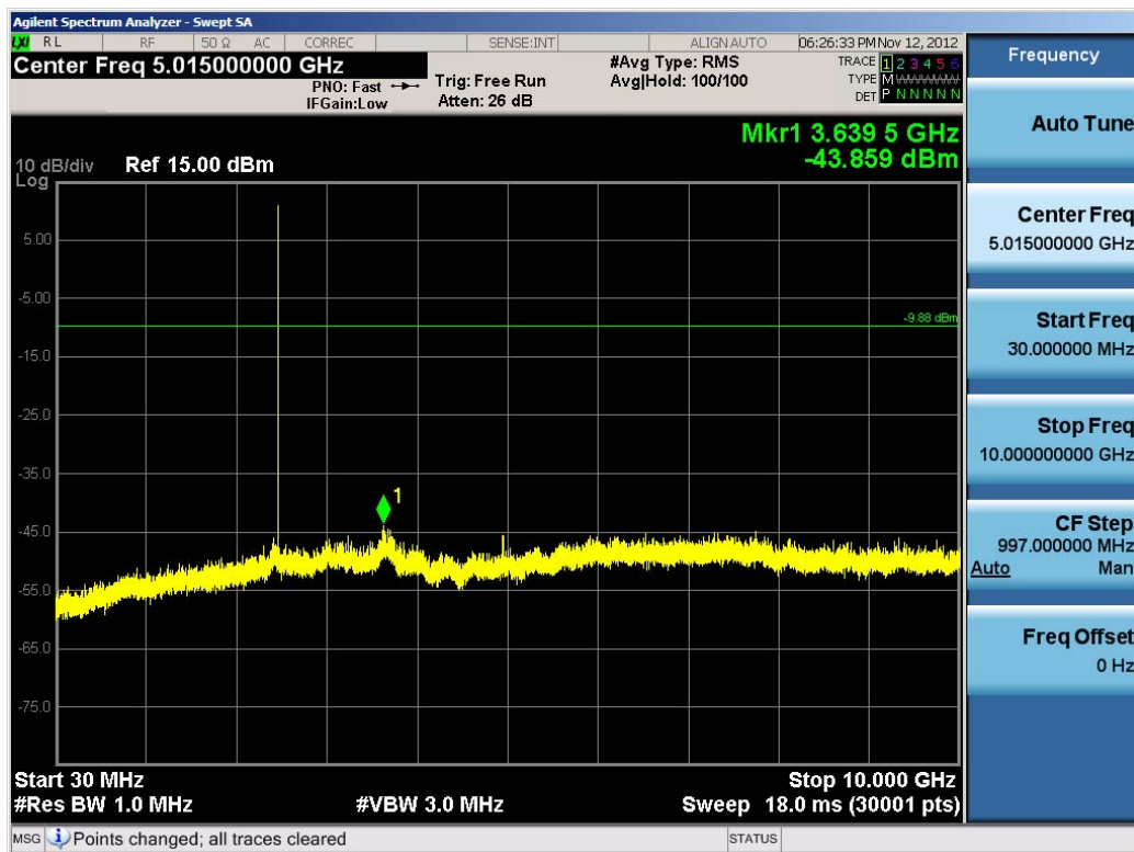
Plot 6-31. Conducted Spurious Plot (Bluetooth, 1Mbps – Ch. 78)
