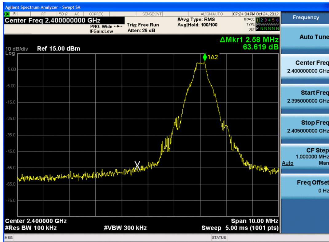
Plot 6-19. Band Edge Plot (Bluetooth with Hopping Disabled, 1Mbps – Ch. 0)
