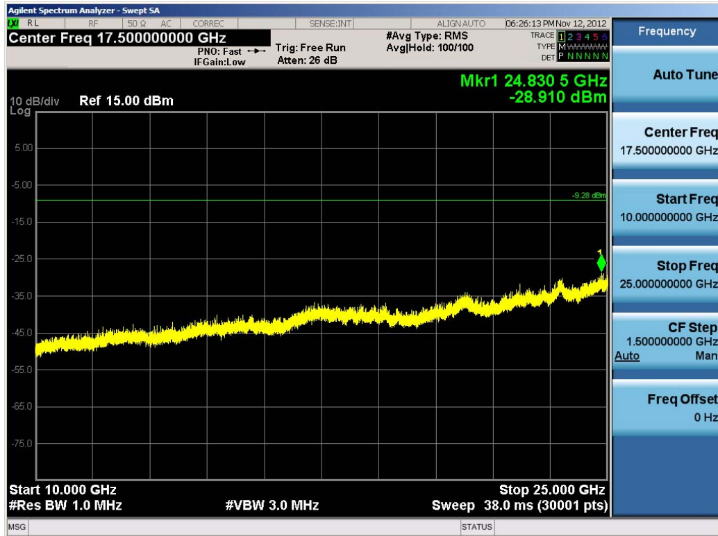
Plot 6-30. Conducted Spurious Plot (Bluetooth, 1Mbps – Ch. 39)
