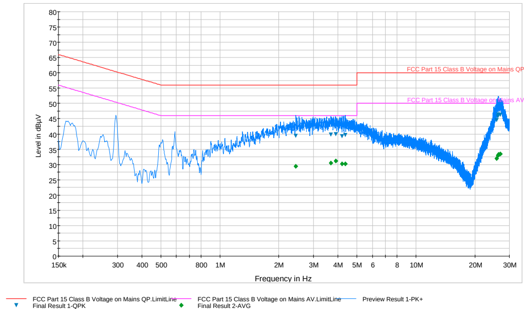
Plot 6-55. Line Conducted Plot with 802.11a UNII Band 1 (N)
