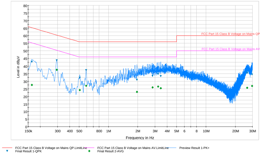
Plot 6-58. Line Conducted Plot with 802.11a UNII Band 3 (L1)
