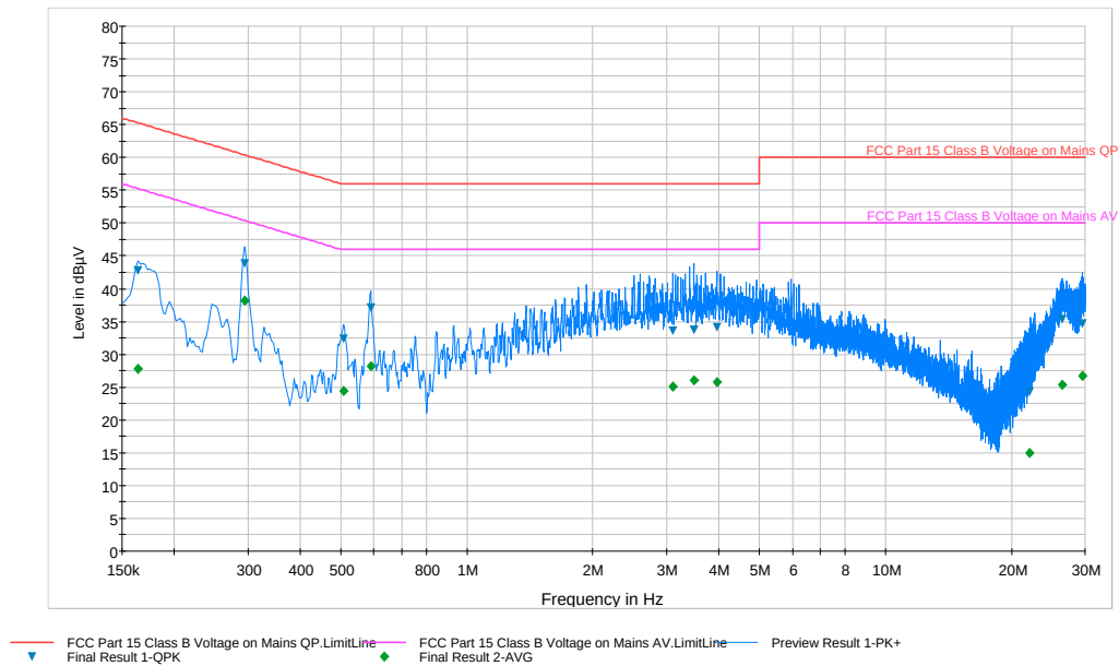
Plot 6-54. Line Conducted Plot with 802.11a UNII Band 1 (L1)
