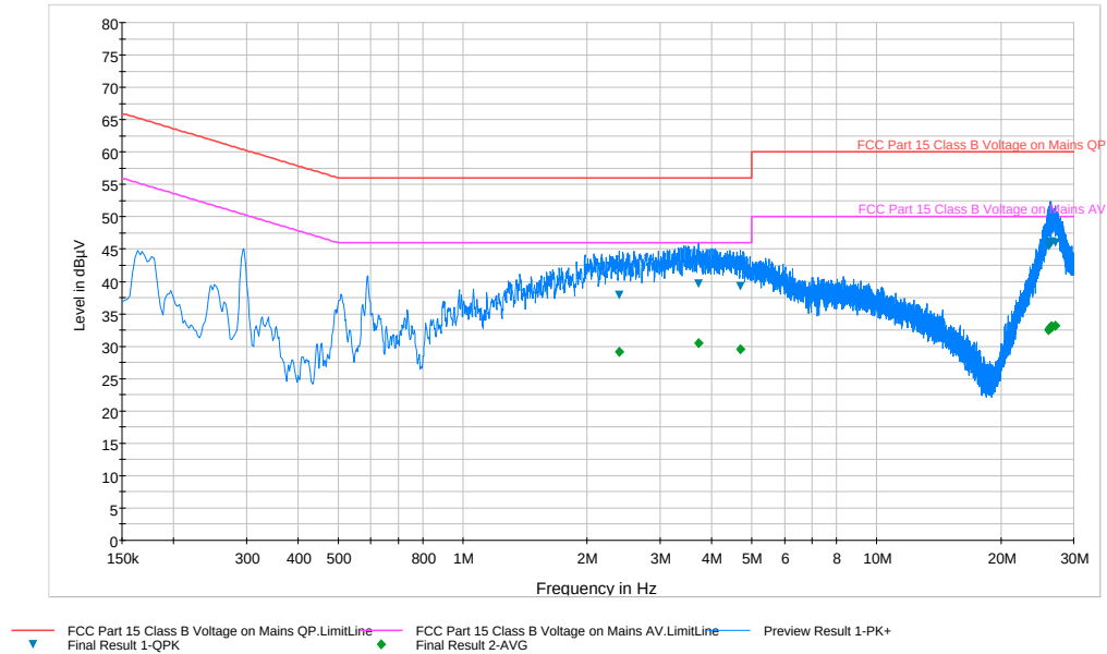
Plot 6-59. Line Conducted Plot with 802.11a UNII Band 3 (N)
