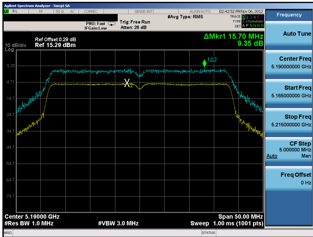
Plot 6-53. Peak Excursion Ratio Plot (40MHz BW 802.11n (UNII Band 1) – Ch. 38)
