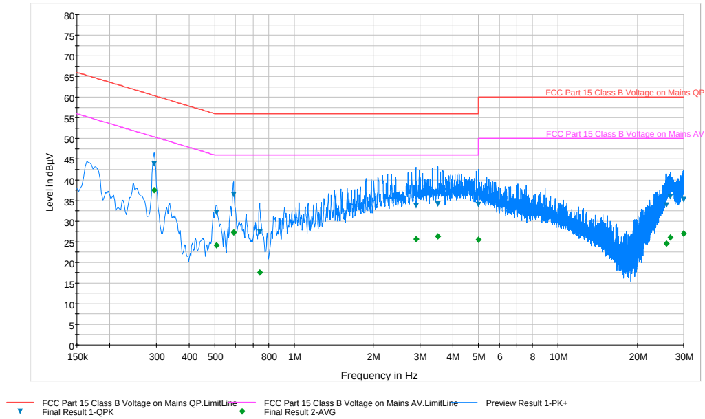
Plot 6-56. Line Conducted Plot with 802.11a UNII Band 2 (L1)
