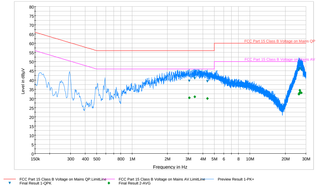
Plot 6-57. Line Conducted Plot with 802.11a UNII Band 2 (N)
