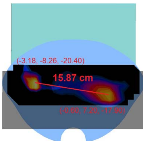
Figure 11-4 Peak SAR Location Plot of GPRS 1900 and 2.4 GHz WLAN for Back Side (at 1.2 cm)
