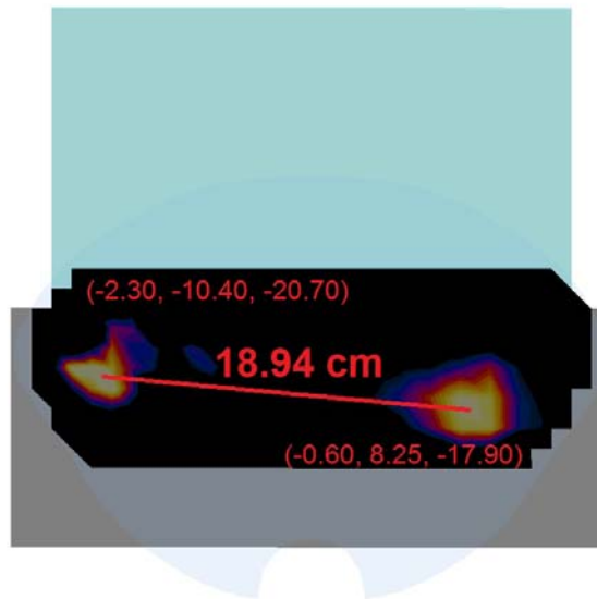
Figure 11-3 Peak SAR Location Plot of UMTS 1900 and 5 GHz WLAN for Back Side (at 0.0 cm)
