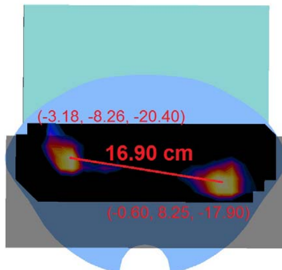
Figure 11-2 Peak SAR Location Plot of UMTS 1900 and 2.4 GHz WLAN for Back Side (at 0.0 cm)
