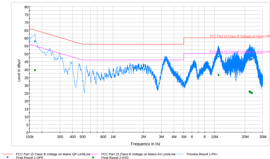
Plot 6-16. Line Conducted Plot with Bluetooth LE (N)
